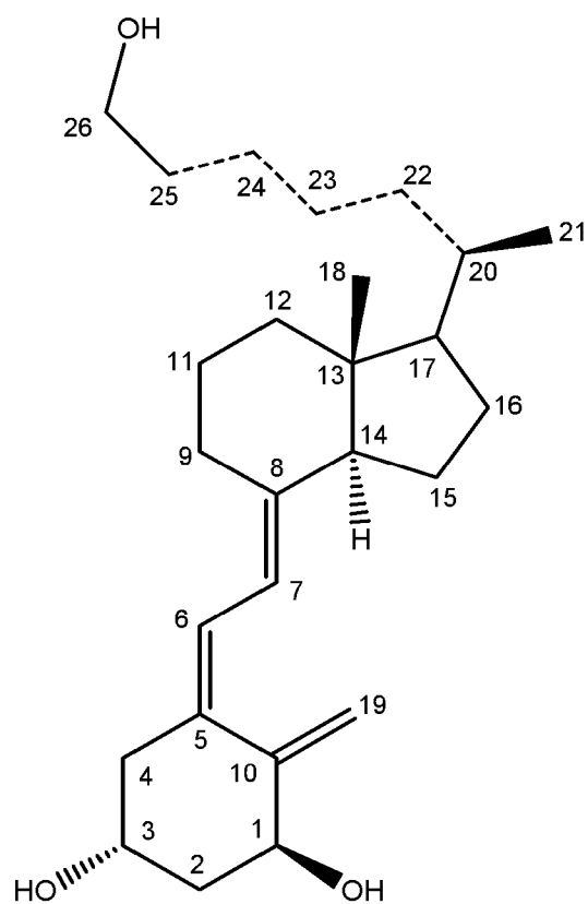
Formula (v)
