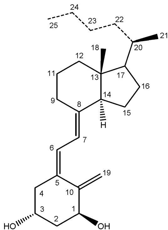
Formula (ii)
