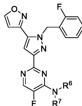
Formula VII
