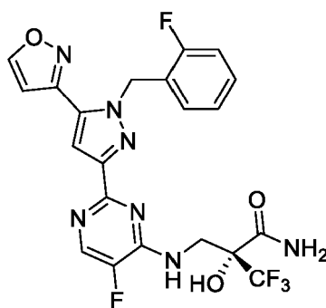
Formula ID
