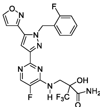
Formula IB
