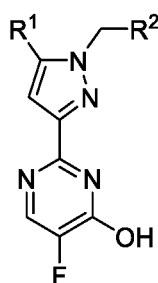
Compound 9
