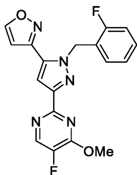
Formula V
