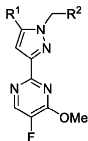
Formula II
