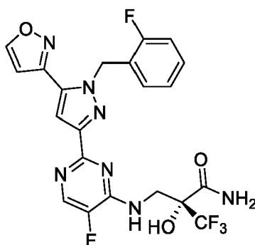
Formula ID
