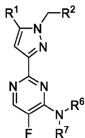
Formula IV
