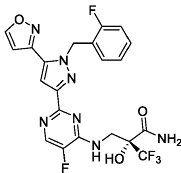
Formula ID
