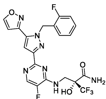
Formula ID
