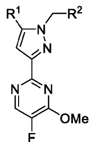
Formula II
