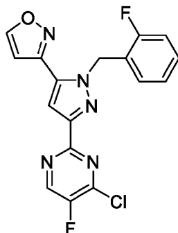
Formula VI
