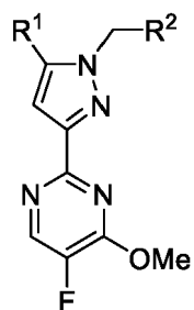
Formula II
