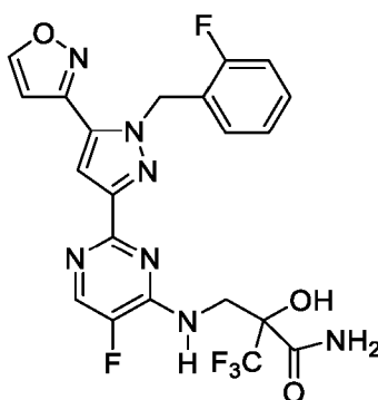
Formula IB
