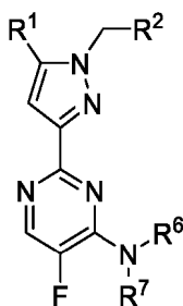
Formula IV
