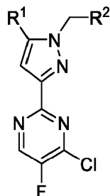
Formula III
