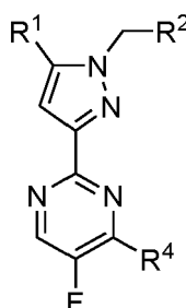
Formula I
