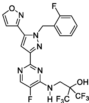
Formula IA
