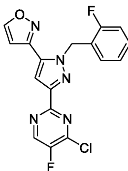
Formula VI
