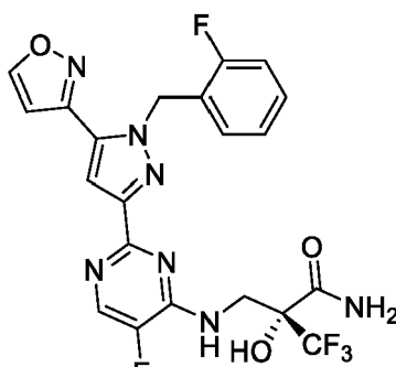
Formula ID
