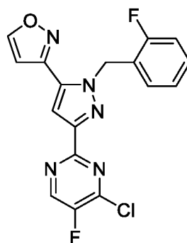
Formula VI
