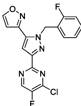
Formula VI
