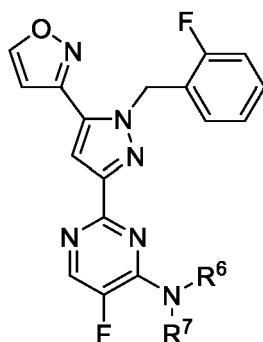
Formula VII
