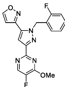
Formula V
