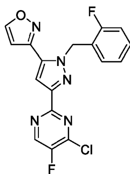
Formula VI
