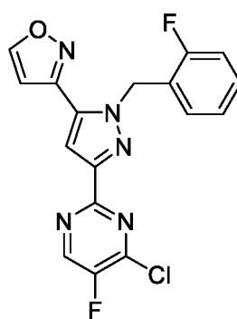
Formula VI
