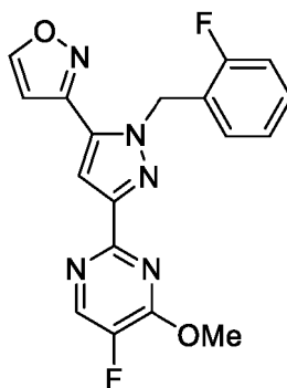
Formula V
