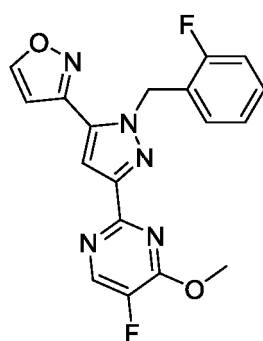
Formula V
