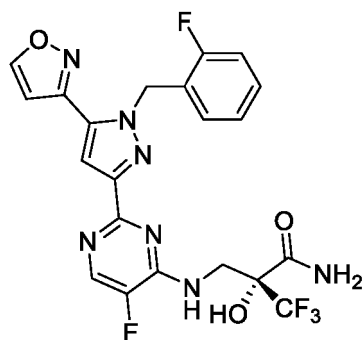
Formula ID
