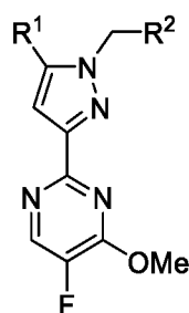
Formula II
