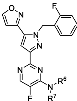
Formula VII
