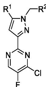
Formula III
