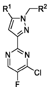
Formula III
