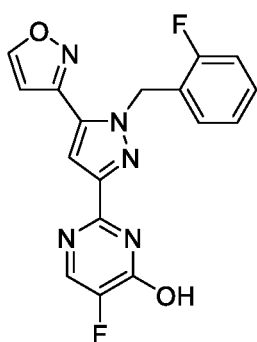
Compound 9'
