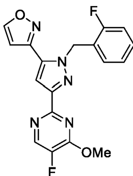
Formula V
