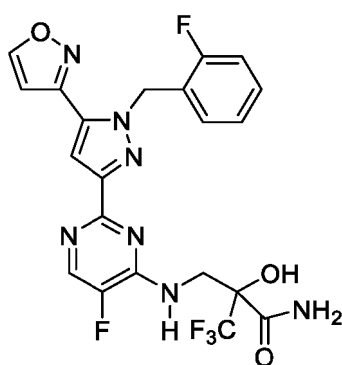
Formula IB
