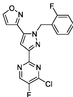
Formula VI
