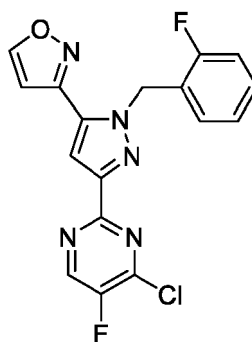
Formula VI
