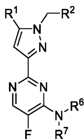
Formula IV
