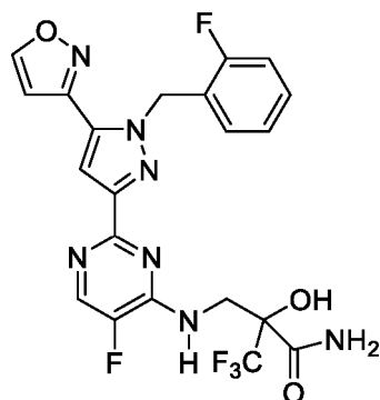
Formula IB
