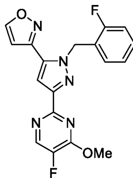
Formula V
