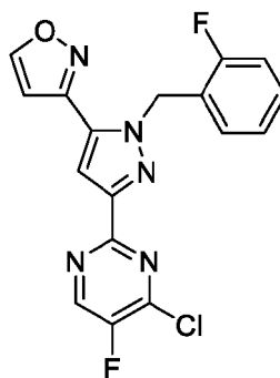
Formula VI
