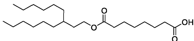
8-((3-Hexylnonyl)oxy)-8-oxooctanoic acid
