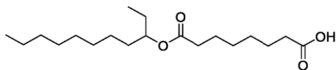
8-Oxo-8-(undecan-3-yloxy)octanoic acid
