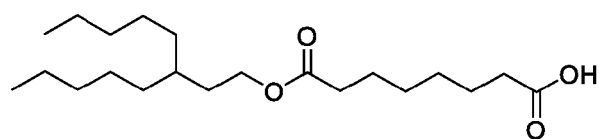
8-Oxo-8-((3-pentyloctyl)oxy)octanoic acid
