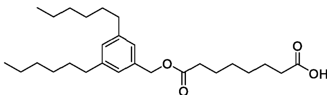
8-((3,5-Dihexylbenzyl)oxy)-8-oxooctanoic acid
