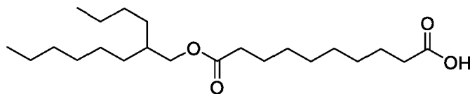
10-((2-Butyloctyl)oxy)-10-oxodecanoic acid
