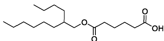
6-((2-Butyloctyl)oxy)-6-oxohexanoic acid
