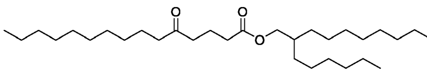
2-Hexyldecyl 5-oxopentadecanoate
