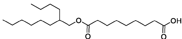
9-((2-Butyloctyl)oxy)-9-oxononanoic acid
