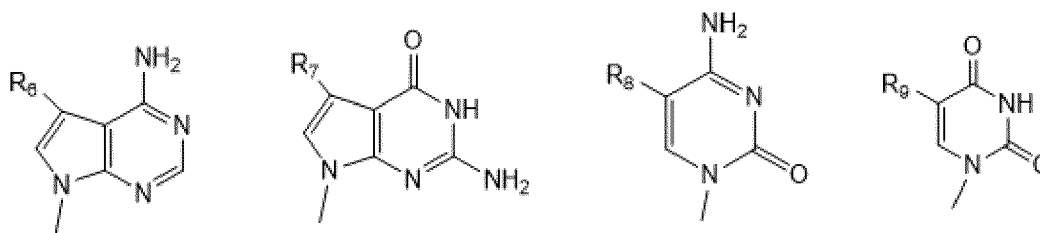
STRUCTURES XV-XVIII
