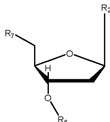
Structure IV
