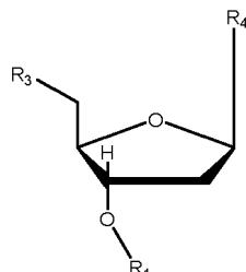
Structure II
