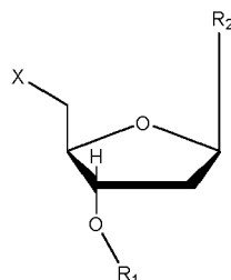
Structure III
