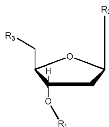
Structure I
