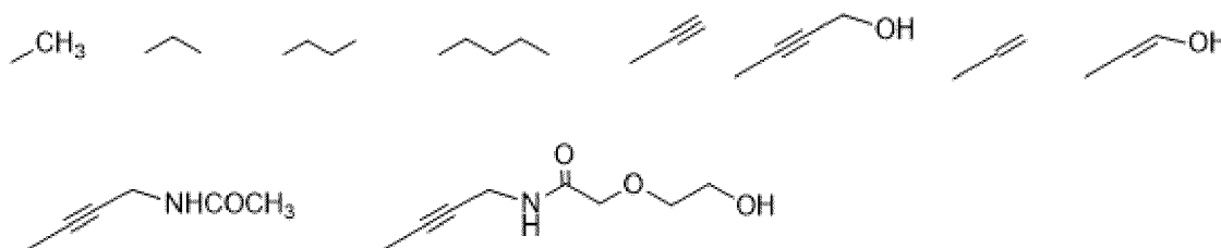
STRUCTURES XIX-XXVIII
