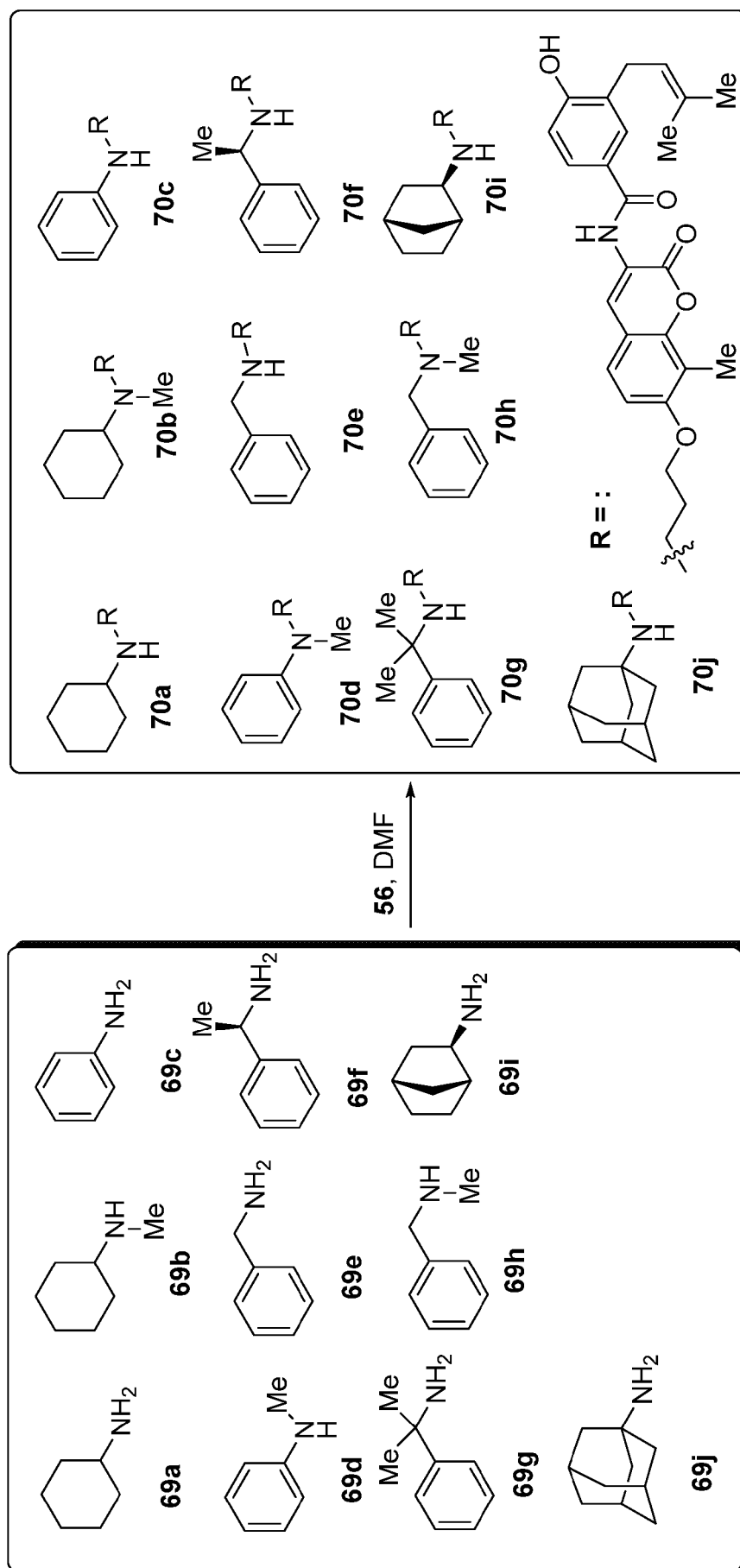
Scheme 9: Synthesis of Alkylamine Derivatives with Cyclic N-substitutions
