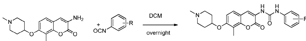
Scheme 1: General Urea Synthesis Methodology
