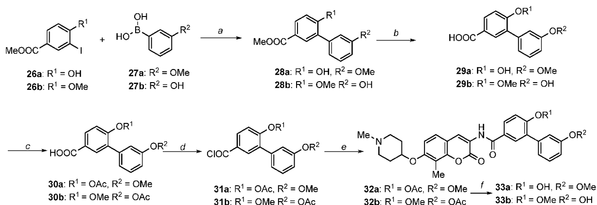
Scheme 5: Synthesis of Biphenyl Substituted Amide
