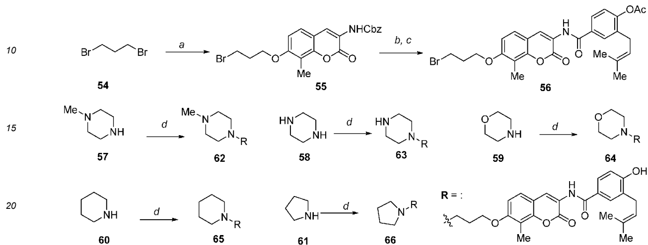
Scheme 7: Synthesis of Terminal Cycloamine Derivatives of Novobiocin
