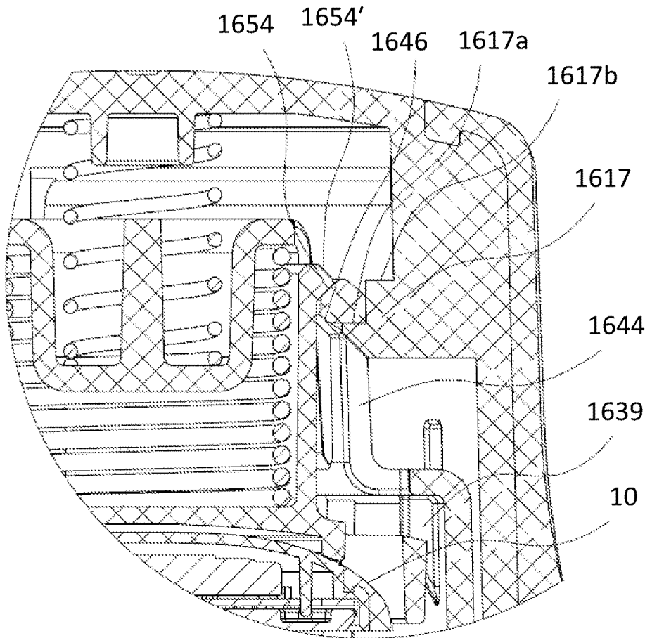
DETAIL C SCALE 3 : 1
