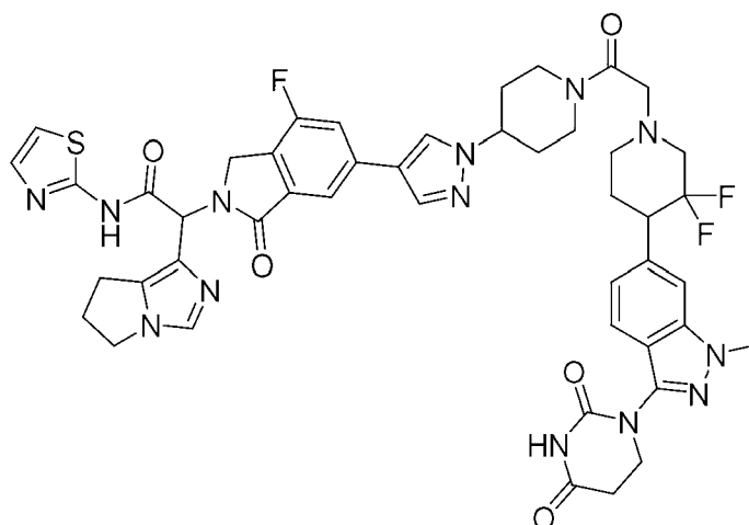
2-(6,7-dihydro-5H-pyrrolo[1,2-c]imidazol-1-yl)-2-(6-(1-(1-(2-(4-(3-(2,4-dioxotetrahydropyrimidin-1(2H)-yl)-1-methyl-1H-indazol-6-yl)-3,3-difluoropiperidin-1-yl)acetyl)piperidin-4-yl)-1H-pyrazol-4-yl)-4-fluoro-1-oxoisindolin-2-yl)-N-(thiazol-2-yl)acetamide
