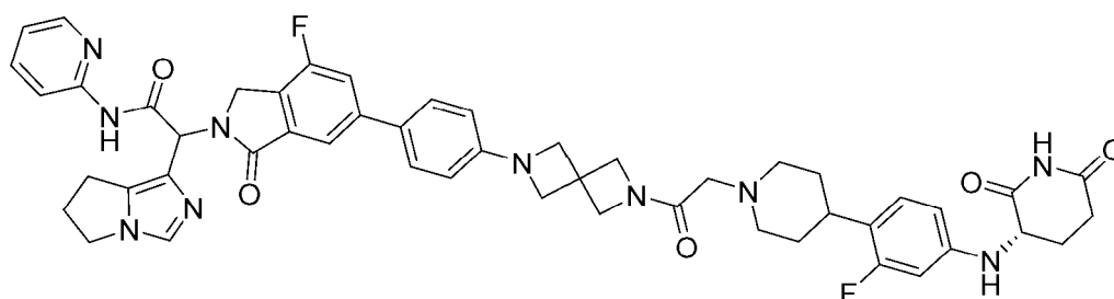
2-(6,7-dihydro-5H-pyrrolo[1,2-c]imidazol-1-yl)-2-[6-[4-[2-[2-[4-[4-[(3S)-2,6-dioxo-3-piperidyl]amino]-2-fluoro-phenyl]-1-piperidyl]acetyl]-2,6-diazaspiro[3.3]heptan-6-yl]phenyl]-4-fluoro-1-oxo-isindolin-2-yl]-N-(2-pyridyl)acetamide
