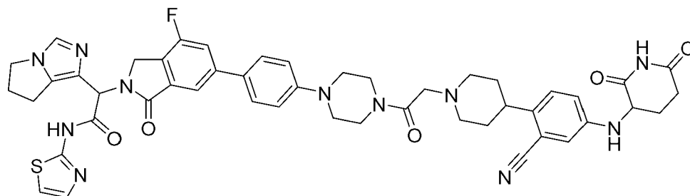
2-[6-[4-[4-[2-[4-[2-cyano-4-[(2,6-dioxo-3-piperidyl)amino]phenyl]-1-piperidyl]acetyl]piperazin-1-yl]phenyl]-4-fluoro-1-oxo-isoindolin-2-yl]-2-(6,7-dihydro-5H-pyrrolo[1,2-c]imidazol-1-yl)-N-thiazol-2-yl-acetamide
