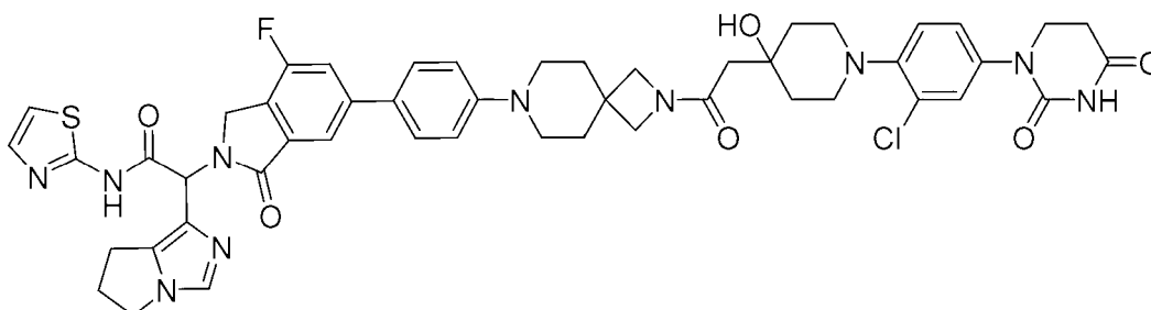
2-[6-[4-[2-[2-[1-[2-chloro-4-(2,4-dioxohexahydropyrimidin-1-yl)phenyl]-4-hydroxy-4-piperidyl]acetyl]-2,7-diazaspiro[3.5]nonan-7-yl]phenyl]-4-fluoro-1-oxo-isoindolin-2-yl]-2-(6,7-dihydro-5H-pyrrolo[1,2-c]imidazol-1-yl)-N-thiazol-2-yl-acetamide
