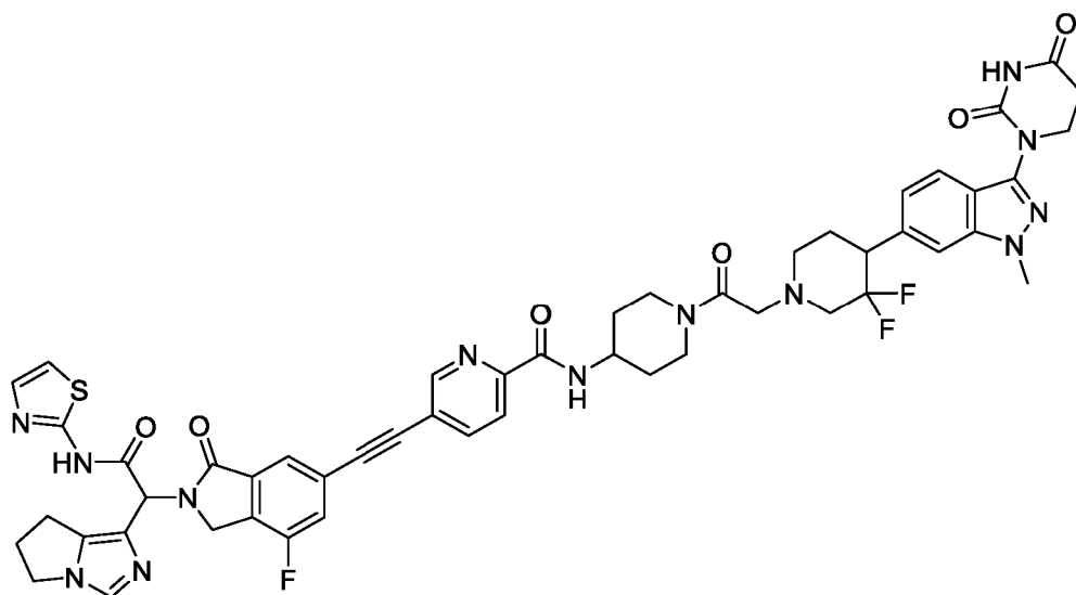
5-((2-(1-(6,7-dihydro-5H-pyrrolo[1,2-c]imidazol-1-yl)-2-oxo-2-(thiazol-2-ylamino)ethyl)-7-fluoro-3-oxoisindolin-5-yl)ethynyl)-N-(1-(2-(4-(3-(2,4-dioxotetrahydropyrimidin-1(2H)-yl)-1-methyl-1H-indazol-6-yl)-3,3-difluoropiperidin-1-yl)acetyl)piperidin-4-yl)picolinamide
