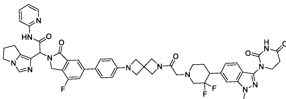
2-(6,7-dihydro-5H-pyrrolo[1,2-c]imidazol-1-yl)-2-[6-[4-[2-[2-[4-[3-(2,4-dioxohexahydropyrimidin-1-yl)-1-methyl-indazol-6-yl]-3,3-difluoro-1-piperidyl]acetyl]-2,6-diazaspiro[3.3]heptan-6-yl]phenyl]-4-fluoro-1-oxo-isindolin-2-yl]-N-(2-pyridyl)acetamide
