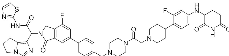
2-(6,7-dihydro-5H-pyrrolo[1,2-c]imidazol-1-yl)-2-[6-[4-[4-[2-[4-[4-[(2,6-dioxo-3-piperidyl)amino]-2-fluoro-phenyl]-1-piperidyl]acetyl]piperazin-1-yl]methyl]phenyl]-4-fluoro-1-oxo-isindolin-2-yl]-N-thiazol-2-yl-acetamide
