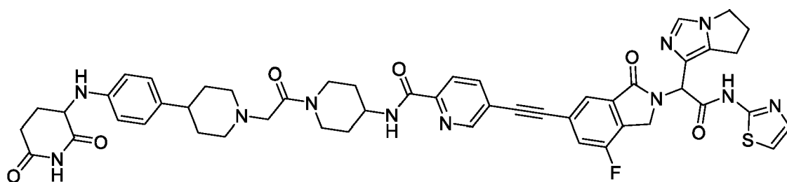
5-((2-(1-(6,7-dihydro-5H-pyrrolo[1,2-c]imidazol-1-yl)-2-oxo-2-(thiazol-2-ylamino)ethyl)-7-fluoro-3-oxoisoindolin-5-yl)ethynyl)-N-(1-(2-(4-(4-((2,6-dioxopiperidin-3-yl)amino)phenyl)piperidin-1-yl)acetyl)piperidin-4-yl)picolinamide;
