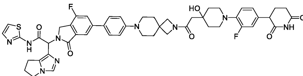
2-(6,7-dihydro-5H-pyrrolo[1,2-c]imidazol-1-yl)-2-[6-[4-[2-[2-[1-[4-(2,6-dioxo-3-piperidyl)-2-fluoro-phenyl]-4-hydroxy-4-piperidyl]acetyl]-2,7-diazaspiro[3.5]nonan-7-yl]phenyl]-4-fluoro-1-oxo-isoindolin-2-yl]-N-thiazol-2-yl-acetamide
