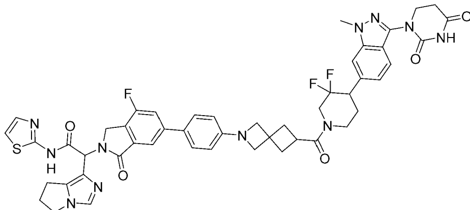
2-(6,7-dihydro-5H-pyrrolo[1,2-c]imidazol-1-yl)-2-[6-[4-[6-[4-[3-(2,4-dioxohexahydropyrimidin-1-yl)-1-methyl-indazol-6-yl]-3,3-difluoro-piperidine-1-carbonyl]-2-azaspiro[3.3]heptan-2-yl]phenyl]-4-fluoro-1-oxo-isoindolin-2-yl]-N-thiazol-2-yl-acetamide
