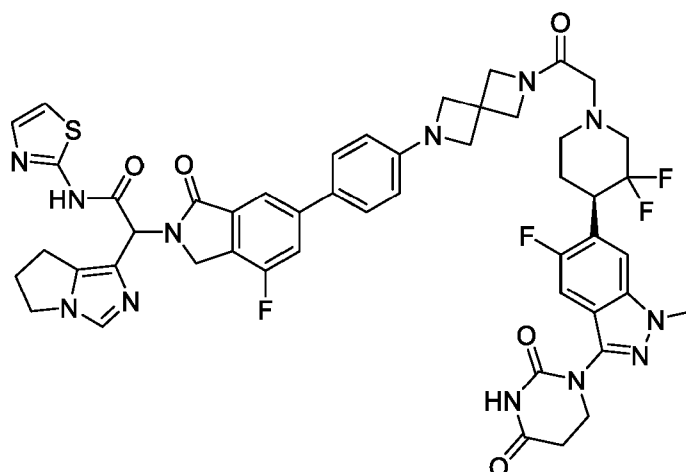
2-(6,7-dihydro-5H-pyrrolo[1,2-c]imidazol-1-yl)-2-(6-(4-(6-(2-((R)-4-(3-(2,4-dioxotetrahydropyrimidin-1(2H)-yl)-5-fluoro-1-methyl-1H-indazol-6-yl)-3,3-
