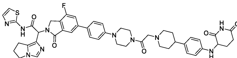
2-(6,7-dihydro-5H-pyrrolo[1,2-c]imidazol-1-yl)-2-[6-[4-[4-[2-[4-[4-[(2,6-dioxo-3-piperidyl)amino]phenyl]-1-piperidyl]acetyl]piperazin-1-yl]phenyl]-4-fluoro-1-oxo-isoindolin-2-yl]-N-thiazol-2-yl-acetamide
