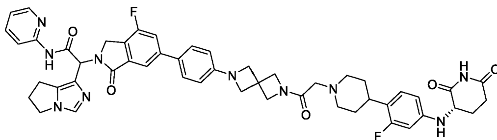
2-(6,7-dihydro-5H-pyrrolo[1,2-c]imidazol-1-yl)-2-[6-[4-[2-[2-[4-[4-[(3S)-2,6-dioxo-3-piperidyl]amino]-2-fluoro-phenyl]-1-piperidyl]acetyl]-2,6-diazaspiro[3.3]heptan-6-yl]phenyl]-4-fluoro-1-oxo-isindolin-2-yl]-N-(2-pyridyl)acetamide
