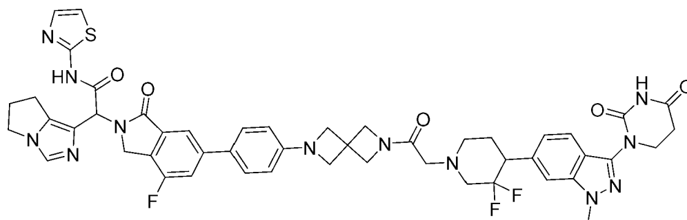
2-(6,7-dihydro-5H-pyrrolo[1,2-c]imidazol-1-yl)-2-[6-[4-[2-[2-[4-[3-(2,4-dioxohexahydropyrimidin-1-yl)-1-methyl-indazol-6-yl]-3,3-difluoro-1-piperidyl]acetyl]-2,6-diazaspiro[3.3]heptan-6-yl]phenyl]-4-fluoro-1-oxo-isindolin-2-yl]-N-thiazol-2-yl-acetamide
