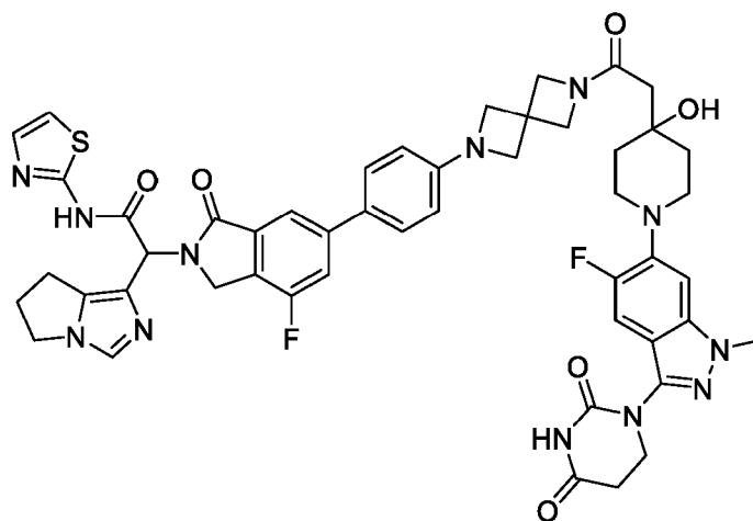
2-(6,7-dihydro-5H-pyrrolo[1,2-c]imidazol-1-yl)-2-(6-(4-(6-(2-(1-(3-(2,4-dioxotetrahydropyrimidin-1(2H)-yl)-5-fluoro-1-methyl-1H-indazol-6-yl)-4-hydroxypiperidin-4-yl)acetyl)-2,6-diazaspiro[3.3]heptan-2-yl)phenyl)-4-fluoro-1-oxoisindolin-2-yl)-N-(thiazol-2-yl)acetamide
