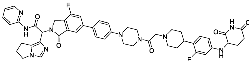
2-(6,7-dihydro-5H-pyrrolo[1,2-c]imidazol-1-yl)-2-[6-[4-[4-[2-[4-[4-[(2,6-dioxo-3-piperidyl)amino]-2-fluoro-phenyl]-1-piperidyl]acetyl]piperazin-1-yl]phenyl]-4-fluoro-1-oxo-isindolin-2-yl]-N-(2-pyridyl)acetamide
