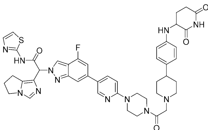
2-(6,7-dihydro-5H-pyrrolo[1,2-c]imidazol-1-yl)-2-[6-[6-[4-[2-[4-[4-[(2,6-dioxo-3-piperidyl)amino]phenyl]-1-piperidyl]acetyl]piperazin-1-yl]-3-pyridyl]-4-fluoro-indazol-2-yl]-N-thiazol-2-yl-acetamide
