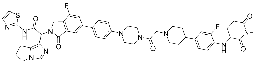
2-(6,7-dihydro-5H-pyrrolo[1,2-c]imidazol-1-yl)-2-[6-[4-[4-[2-[4-[4-[(2,6-dioxo-3-piperidyl)amino]-3-fluoro-phenyl]-1-piperidyl]acetyl]piperazin-1-yl]phenyl]-4-fluoro-1-oxo-isoindolin-2-yl]-N-thiazol-2-yl-acetamide
