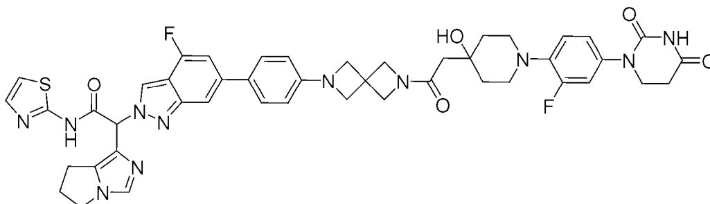
2-(6,7-dihydro-5H-pyrrolo[1,2-c]imidazol-1-yl)-2-[6-[4-[2-[2-[1-[4-(2,4-dioxohexahydropyrimidin-1-yl)-2-fluoro-phenyl]-4-hydroxy-4-piperidyl]acetyl]-2,6-diazaspiro[3.3]heptan-6-yl]phenyl]-4-fluoro-indazol-2-yl]-N-thiazol-2-yl-acetamide
