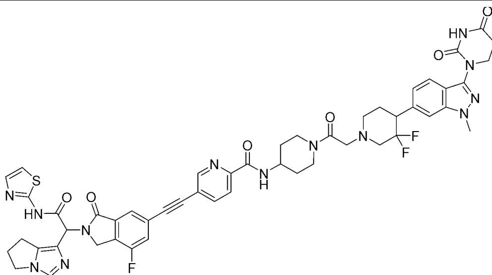
5-((2-(1-(6,7-dihydro-5H-pyrrolo[1,2-c]imidazol-1-yl)-2-oxo-2-(thiazol-2-ylamino)ethyl)-7-fluoro-3-oxoisindolin-5-yl)ethynyl)-N-(1-(2-(4-(3-(2,4-dioxotetrahydropyrimidin-1(2H)-yl)-1-methyl-1H-indazol-6-yl)-3,3-difluoropiperidin-1-yl)acetyl)piperidin-4-yl)picolinamide
