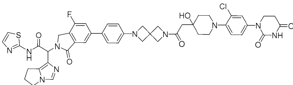
2-[6-[4-[2-[2-[1-[2-chloro-4-(2,4-dioxohexahydropyrimidin-1-yl)phenyl]-4-hydroxy-4-piperidyl]acetyl]-2,6-diazaspiro[3.3]heptan-6-yl]phenyl]-4-fluoro-1-oxo-isoindolin-2-yl]-2-(6,7-dihydro-5H-pyrrolo[1,2-c]imidazol-1-yl)-N-thiazol-2-yl-acetamide
