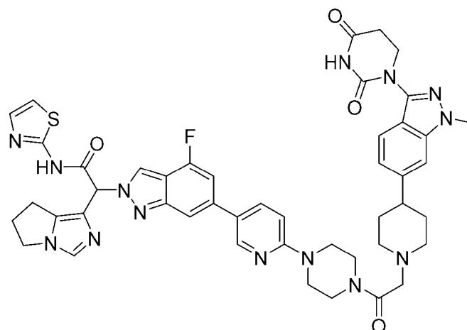
2-(6,7-dihydro-5H-pyrrolo[1,2-c]imidazol-1-yl)-2-[6-[6-[4-[2-[4-[3-(2,4-dioxohexahydropyrimidin-1-yl)-1-methyl-indazol-6-yl]-1-piperidyl]acetyl]piperazin-1-yl]-3-pyridyl]-4-fluoro-indazol-2-yl]-N-thiazol-2-yl-acetamide
