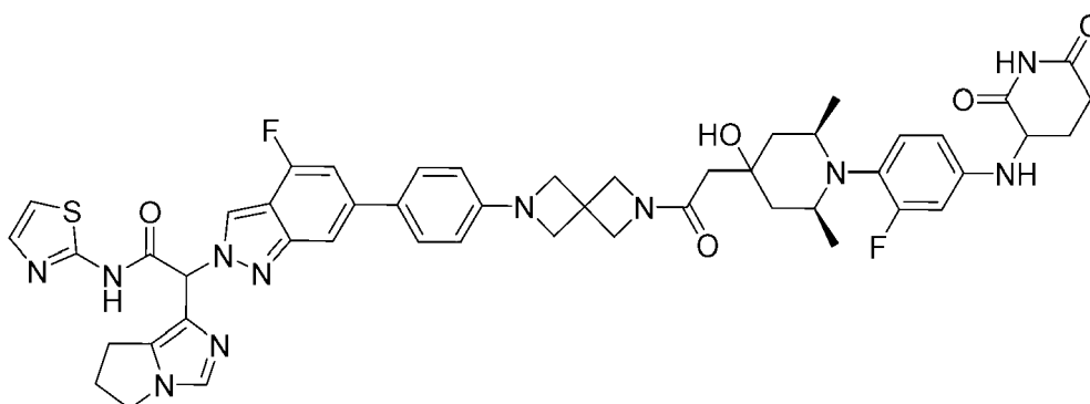
2-(6,7-dihydro-5H-pyrrolo[1,2-c]imidazol-1-yl)-2-[6-[4-[2-[2-[(2s,6r)-1-[4-[(2,6-dioxo-3-piperidyl)amino]-2-fluoro-phenyl]-4-hydroxy-2,6-dimethyl-4-piperidyl]acetyl]-2,6-diazaspiro[3.3]heptan-6-yl]phenyl]-4-fluoro-indazol-2-yl]-N-thiazol-2-yl-acetamide
