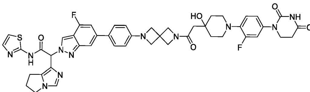
2-(6,7-dihydro-5H-pyrrolo[1,2-c]imidazol-1-yl)-2-[6-[4-[2-[2-[1-[4-(2,4-dioxohexahydropyrimidin-1-yl)-2-fluoro-phenyl]-4-hydroxy-4-piperidyl]acetyl]-2,6-diazaspiro[3.3]heptan-6-yl]phenyl]-4-fluoro-indazol-2-yl]-N-thiazol-2-yl-acetamide
