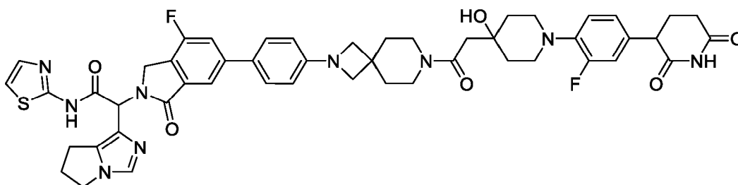
2-(6,7-dihydro-5H-pyrrolo[1,2-c]imidazol-1-yl)-2-[6-[4-[7-[2-[1-[4-(2,6-dioxo-3-piperidyl)-2-fluoro-phenyl]-4-hydroxy-4-piperidyl]acetyl]-2,7-diazaspiro[3.5]nonan-2-yl]phenyl]-4-fluoro-1-oxo-isoindolin-2-yl]-N-thiazol-2-yl-acetamide
