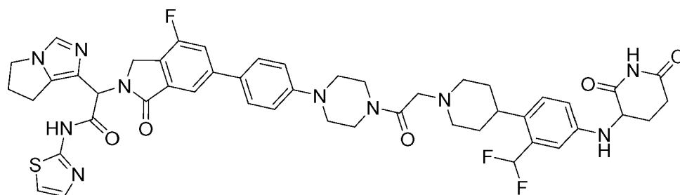
2-[6-[4-[4-[2-[4-[2-(difluoromethyl)-4-[(2,6-dioxo-3-piperidyl)amino]phenyl]-1-piperidyl]acetyl]piperazin-1-yl]phenyl]-4-fluoro-1-oxo-isoindolin-2-yl]-2-(6,7-dihydro-5H-pyrrolo[1,2-c]imidazol-1-yl)-N-thiazol-2-yl-acetamide
