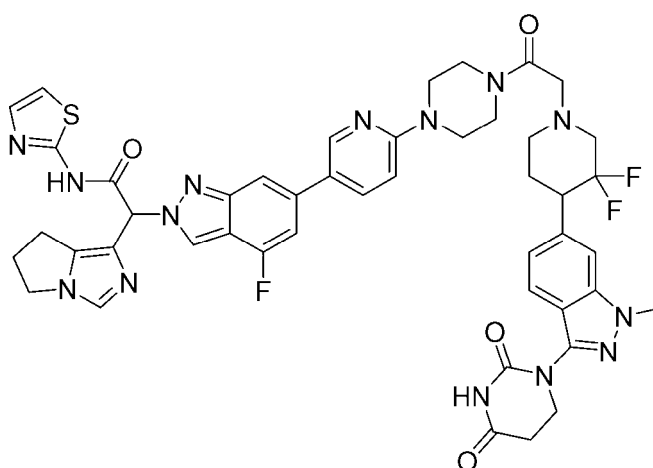
2-(6,7-dihydro-5H-pyrrolo[1,2-c]imidazol-1-yl)-2-(6-(6-(4-(2-(4-(3-(2,4-dioxotetrahydropyrimidin-1(2H)-yl)-1-methyl-1H-indazol-6-yl)-3,3-difluoropiperidin-1-yl)acetyl)piperazin-1-yl)pyridin-3-yl)-4-fluoro-2H-indazol-2-yl)-N-(thiazol-2-yl)acetamide
