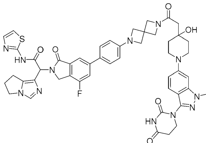
2-(6,7-dihydro-5H-pyrrolo[1,2-c]imidazol-1-yl)-2-(6-(4-(6-(2-(1-(3-(2,4-dioxotetrahydropyrimidin-1(2H)-yl)-1-methyl-1H-indazol-6-yl)-4-hydroxypiperidin-4-yl)acetyl)-2,6-diazaspiro[3.3]heptan-2-yl)phenyl)-4-fluoro-1-oxoisoin-dolin-2-yl)-N-(thiazol-2-yl)acetamide
