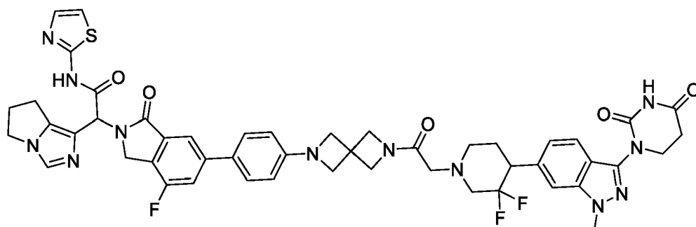
2-(6,7-dihydro-5H-pyrrolo[1,2-c]imidazol-1-yl)-2-[6-[4-[2-[2-[4-[3-(2,4-dioxohexahydropyrimidin-1-yl)-1-methyl-indazol-6-yl]-3,3-difluoro-1-piperidyl]acetyl]-2,6-diazaspiro[3.3]heptan-6-yl]phenyl]-4-fluoro-1-oxo-isindolin-2-yl]-N-thiazol-2-yl-acetamide
