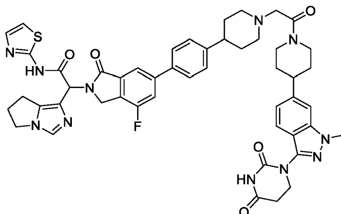
2-(6,7-dihydro-5H-pyrrolo[1,2-c]imidazol-1-yl)-2-(6-(4-(1-(2-(4-(3-(2,4-dioxotetrahydropyrimidin-1(2H)-yl)-1-methyl-1H-indazol-6-yl)piperidin-1-yl)-2-oxoethyl)piperidin-4-yl)phenyl)-4-fluoro-1-oxoisindolin-2-yl)-N-(thiazol-2-yl)acetamide
