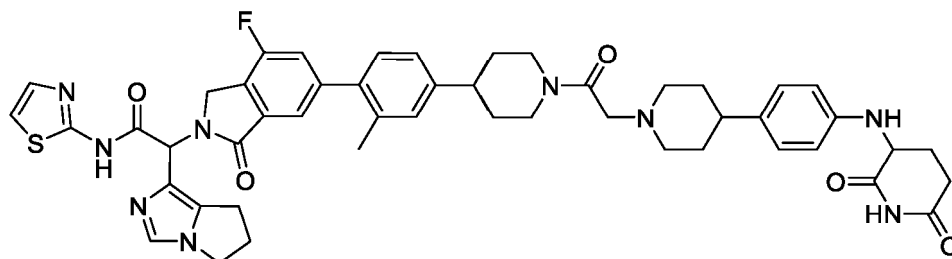
2-(6,7-dihydro-5H-pyrrolo[1,2-c]imidazol-1-yl)-2-[6-[4-[1-[2-[4-[4-[[[(2,6-dioxo-3-piperidyl]amino)]phenyl]-1-piperidyl]acetyl]-4-piperidyl]-2-methyl-phenyl]-4-fluoro-1-oxo-isoindolin-2-yl]-N-thiazol-2-yl]-acetamide
