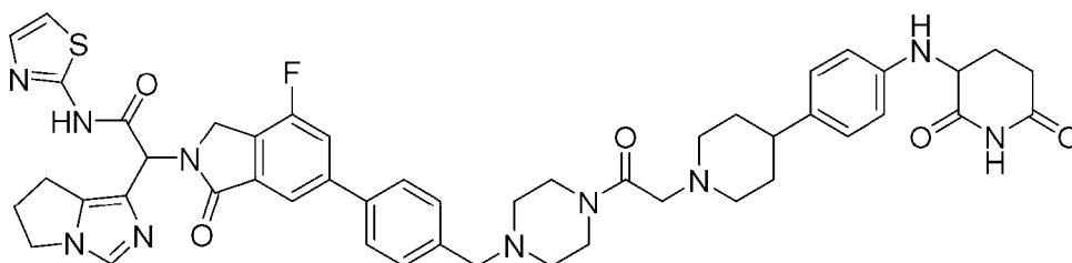
2-(6,7-dihydro-5H-pyrrolo[1,2-c]imidazol-1-yl)-2-[6-[4-[4-[2-[4-[4-[(2,6-dioxo-3-piperidyl)amino]phenyl]-1-piperidyl]acetyl]piperazin-1-yl]methyl]phenyl]-4-fluoro-1-oxo-isindolin-2-yl]-N-thiazol-2-yl-acetamide
