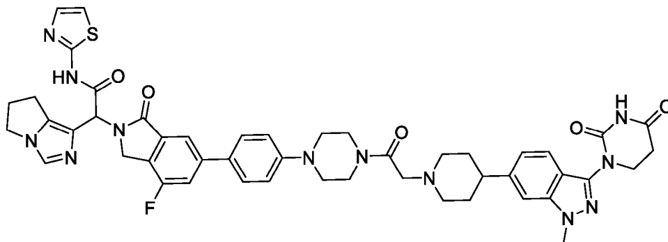
2-(6,7-dihydro-5H-pyrrolo[1,2-c]imidazol-1-yl)-2-(6-(4-(4-(2-(4-(3-(2,4-dioxotetrahydropyrimidin-1(2H)-yl)-1-methyl-1H-indazol-6-yl)piperidin-1-yl)acetyl)piperazin-1-yl)phenyl)-4-fluoro-1-oxoisindolin-2-yl)-N-(thiazol-2-yl)acetamide
