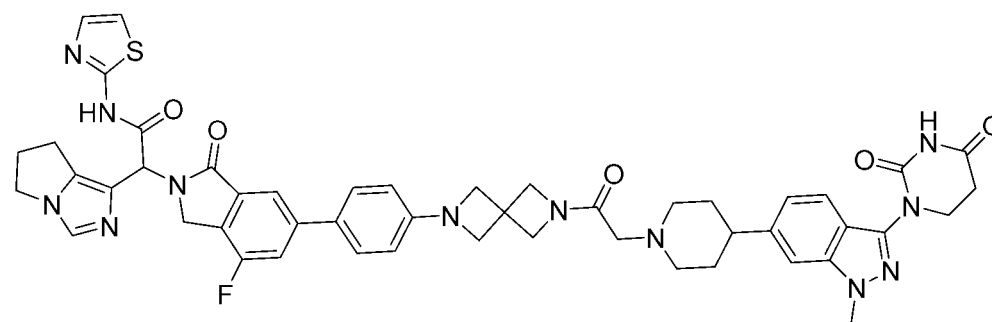
2-(6,7-dihydro-5H-pyrrolo[1,2-c]imidazol-1-yl)-2-[6-[4-[2-[2-[4-[3-(2,4-dioxohexahydropyrimidin-1-yl)-1-methyl-indazol-6-yl]-1-piperidyl]acetyl]-2,6-diazaspiro[3.3]heptan-6-yl]phenyl]-4-fluoro-1-oxo-isindolin-2-yl]-N-thiazol-2-yl-acetamide
