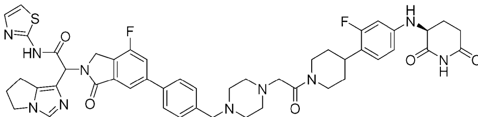
2-(6,7-dihydro-5H-pyrrolo[1,2-c]imidazol-1-yl)-2-[6-[4-[4-[2-[4-[4-[(3S)-2,6-dioxo-3-piperidyl]amino]-2-fluoro-phenyl]-1-piperidyl]-2-oxo-ethyl]piperazin-1-yl]methyl]phenyl]-4-fluoro-1-oxo-isindolin-2-yl]-N-thiazol-2-yl-acetamide
