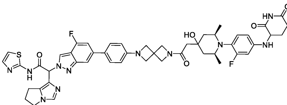
2-(6,7-dihydro-5H-pyrrolo[1,2-c]imidazol-1-yl)-2-[6-[4-[2-[2-[(2S,6R)-1-[4-[(2,6-dioxo-3-piperidyl)amino]-2-fluoro-phenyl]-4-hydroxy-2,6-dimethyl-4-piperidyl]acetyl]-2,6-diazaspiro[3.3]heptan-6-yl]phenyl]-4-fluoro-indazol-2-yl]-N-thiazol-2-yl-acetamide
