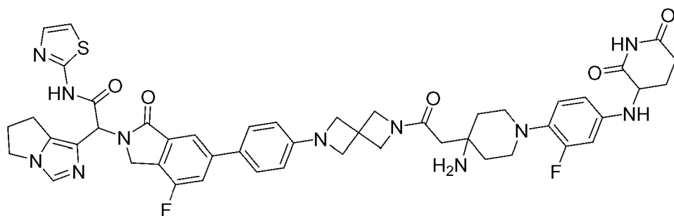
2-[6-[4-[2-[2-[4-amino-1-[4-[(2,6-dioxo-3-piperidyl)amino]-2-fluoro-phenyl]-4-piperidyl]acetyl]-2,6-diazaspiro[3.3]heptan-6-yl]phenyl]-4-fluoro-1-oxo-isoindolin-2-yl]-2-(6,7-dihydro-5H-pyrrolo[1,2-c]imidazol-1-yl)-N-thiazol-2-yl-acetamide
