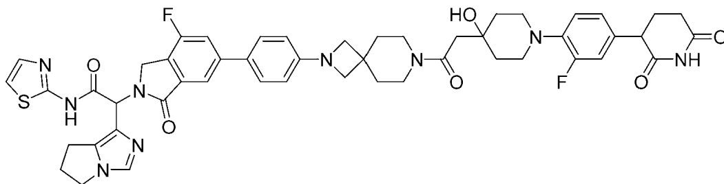
2-(6,7-dihydro-5H-pyrrolo[1,2-c]imidazol-1-yl)-2-[6-[4-[7-[2-[1-[4-(2,6-dioxo-3-piperidyl)-2-fluoro-phenyl]-4-hydroxy-4-piperidyl]acetyl]-2,7-diazaspiro[3.5]nonan-2-yl]phenyl]-4-fluoro-1-oxo-isoindolin-2-yl]-N-thiazol-2-yl-acetamide
