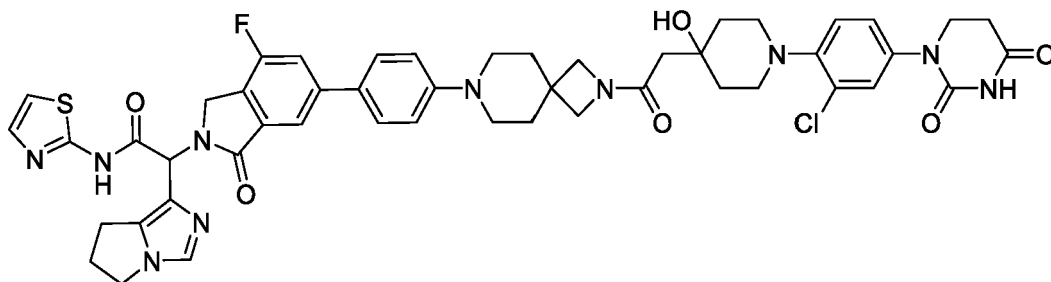
2-[6-[4-[2-[2-[1-[2-chloro-4-(2,4-dioxohexahydropyrimidin-1-yl)phenyl]-4-hydroxy-4-piperidyl]acetyl]-2,7-diazaspiro[3.5]nonan-7-yl]phenyl]-4-fluoro-1-oxo-isoindolin-2-yl]-2-(6,7-dihydro-5H-pyrrolo[1,2-c]imidazol-1-yl)-N-thiazol-2-yl-acetamide
