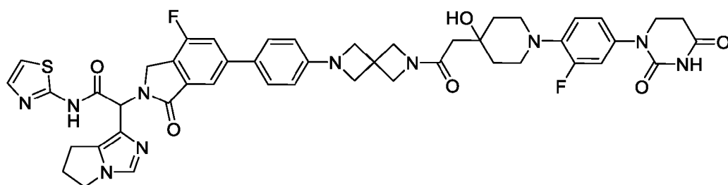
2-(6,7-dihydro-5H-pyrrolo[1,2-c]imidazol-1-yl)-2-[6-[4-[2-[2-[1-[4-(2,4-dioxohexahydropyrimidin-1-yl)-2-fluoro-phenyl]-4-hydroxy-4-piperidyl]acetyl]-2,6-diazaspiro[3.3]heptan-6-yl]phenyl]-4-fluoro-1-oxo-isoindolin-2-yl]-N-thiazol-2-yl-acetamide
