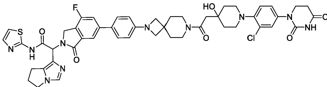
2-[6-[4-[7-[2-[1-[2-chloro-4-(2,4-dioxohexahydropyrimidin-1-yl)phenyl]-4-hydroxy-4-piperidyl]acetyl]-2,7-diazaspiro[3.5]nonan-2-yl]phenyl]-4-fluoro-1-oxo-isoindolin-2-yl]-2-(6,7-dihydro-5H-pyrrolo[1,2-c]imidazol-1-yl)-N-thiazol-2-yl-acetamide
