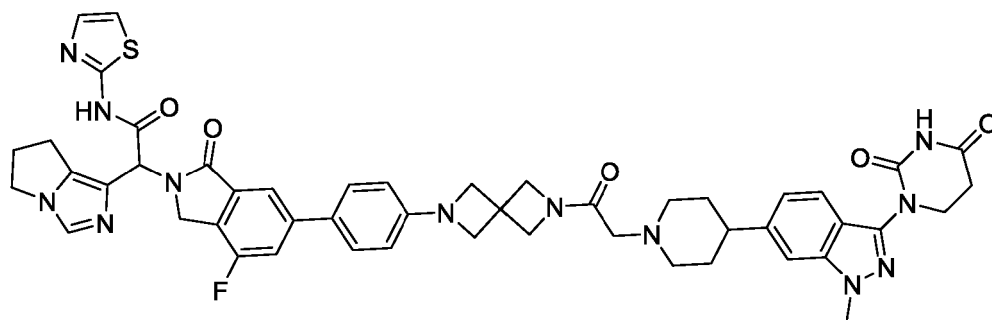
2-(6,7-dihydro-5H-pyrrolo[1,2-c]imidazol-1-yl)-2-[6-[4-[2-[2-[4-[3-(2,4-dioxohexahydropyrimidin-1-yl)-1-methyl-indazol-6-yl]-1-piperidyl]acetyl]-2,6-diazaspiro[3.3]heptan-6-yl]phenyl]-4-fluoro-1-oxo-isindolin-2-yl]-N-thiazol-2-yl-acetamide
