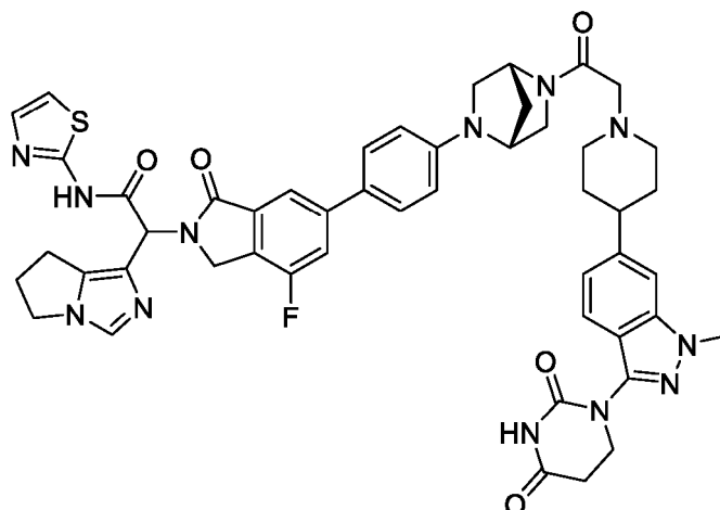
2-(6,7-dihydro-5H-pyrrolo[1,2-c]imidazol-1-yl)-2-(6-(4-((1R,4R)-5-(2-(4-(3-(2,4-dioxotetrahydropyrimidin-1(2H)-yl)-1-methyl-1H-indazol-6-yl)piperidin-1-yl)acetyl)-2,5-diazabicyclo[2.2.1]heptan-2-yl)phenyl)-4-fluoro-1-oxoisindolin-2-yl)-N-(thiazol-2-yl)acetamide
