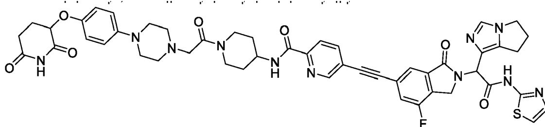
5-[2-[2-[1-(6,7-dihydro-5H-pyrrolo[1,2-c]imidazol-1-yl)-2-oxo-2-(thiazol-2-ylamino)ethyl]-7-fluoro-3-oxo-isoindolin-5-yl]ethynyl]-N-[1-[2-[4-[(2,6-dioxo-3-piperidyl)oxy]phenyl]piperazin-1-yl]acetyl]-4-piperidyl]pyridine-2-carboxamide
