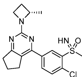
Example 727: (2-chloro-5-(2-((S)-2-methylazetidin-1-yl)-6,7-dihydro-5H-cyclopenta[d]pyrimidin-4-yl)phenyl)(imino)(methyl)-λ 6 -sulfanone
