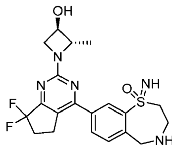
Example 725: 8-(7,7-difluoro-2-((2S,3R)-3-hydroxy-2-methylazetidin-1-yl)-6,7-dihydro-5H-cyclopenta[d]pyrimidin-4-yl)-1-imino-2,3,4,5-tetrahydro-1H-1λ 4 -benzo[f][1,4]thiazepine 1-oxide
