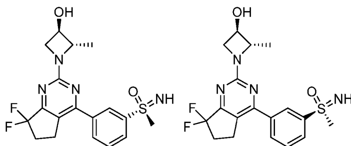
Example 492: (S)-3-(7,7-difluoro-2-((2S,3R)-3-hydroxy-2-methylazetidin-1-yl)-6,7-dihydro-5H-cyclopenta[d]pyrimidin-4-yl)phenyl(imino)(methyl)-λ 6 -sulfanone
