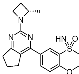
Example 726: 4-imino-6-(2-((S)-2-methylazetidin-1-yl)-6,7-dihydro-5H-cyclopenta[d]pyrimidin-4-yl)-3,4-dihydro-2H-4λ 4 -benzo[b][1,4]oxathiine 4-oxide
