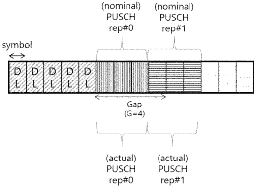
(b) L=3, S=5, K=2 (gap symbol used)
