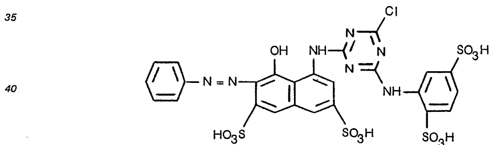
45 1-hydroxy-2-phenylazo-8-[2-chloro-4-(2,5-disulfoanilino)-S-triazine-6-ylamino]naphthalene-3,6-disulfonic acid
