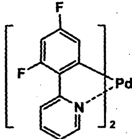
Pd-2
