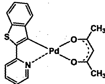
Pd-3
