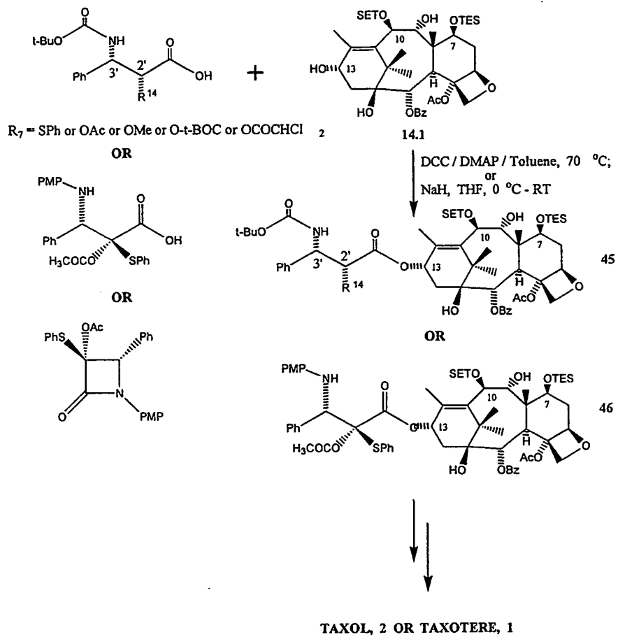
SCHEME 14
