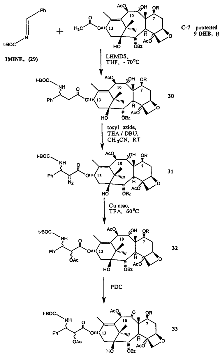
SCHEME 8
