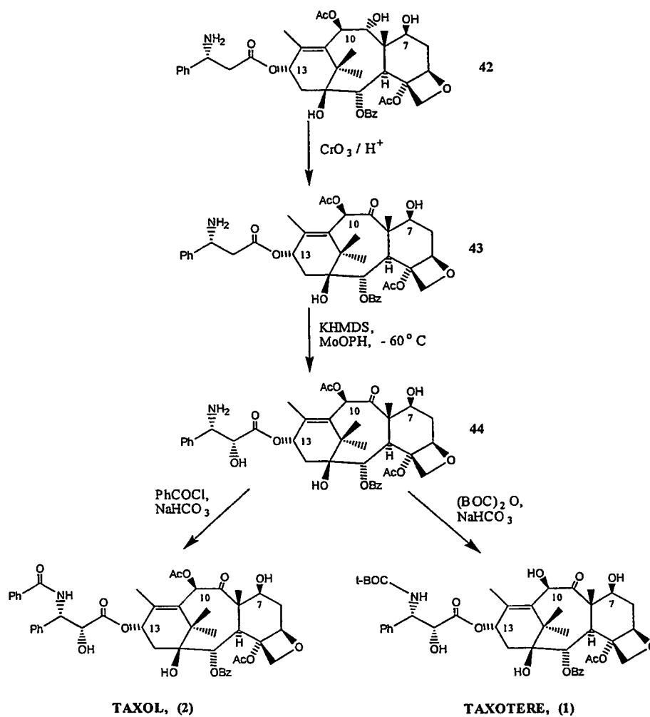
SCHEME 13
