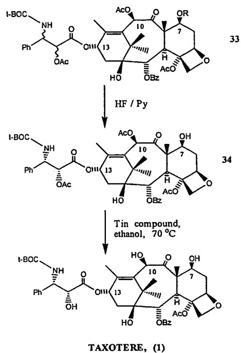
SCHEME 9
