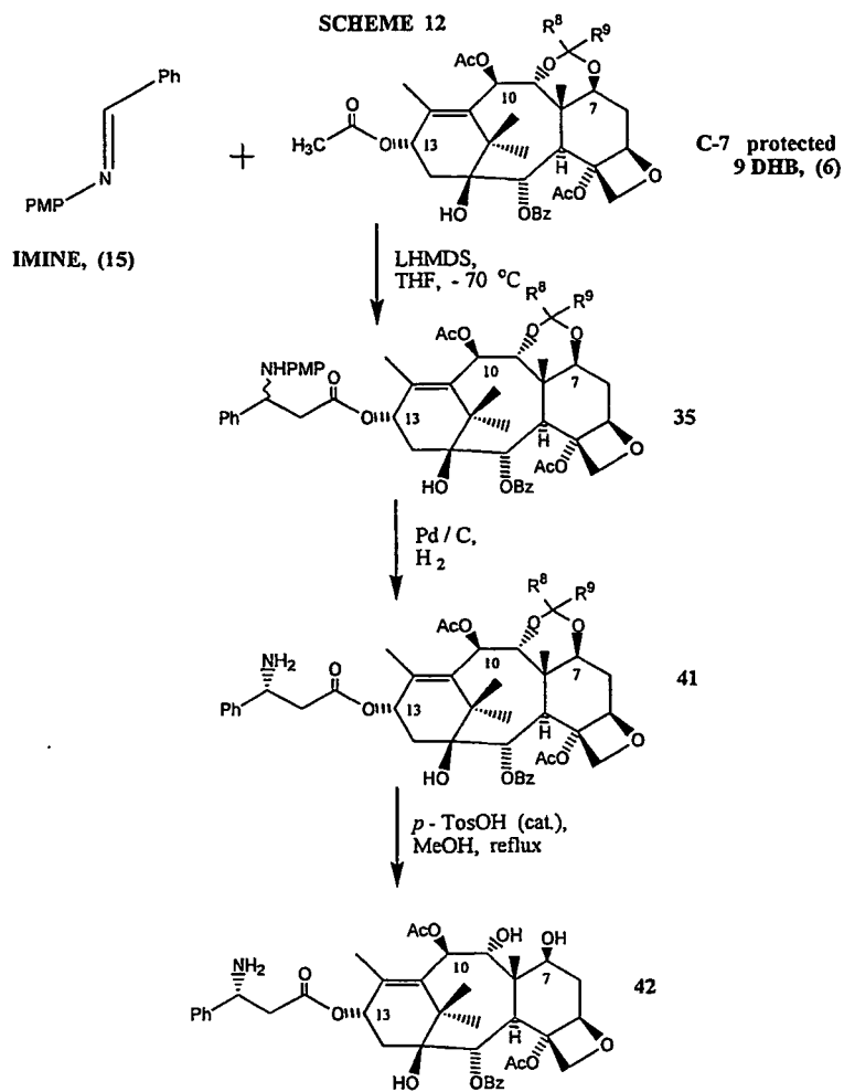
SCHEME 12
