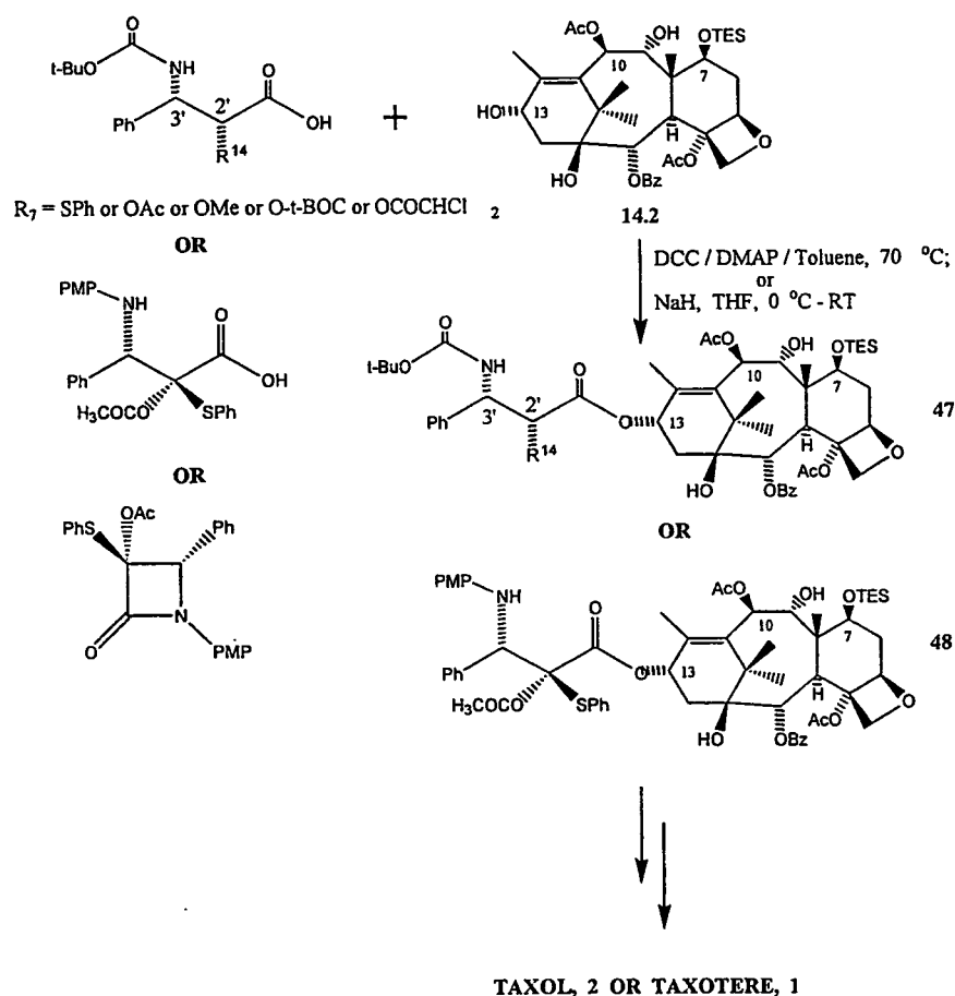
SCHEME 15
