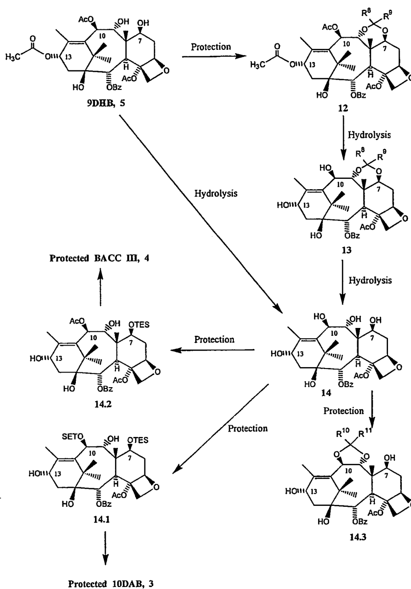
SCHEME 3
