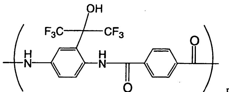
POLYMER (A)
