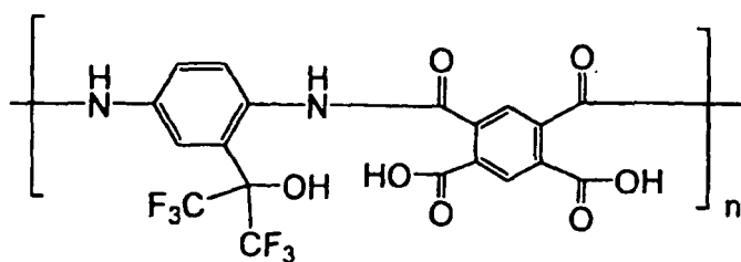
POLYMER (E)
