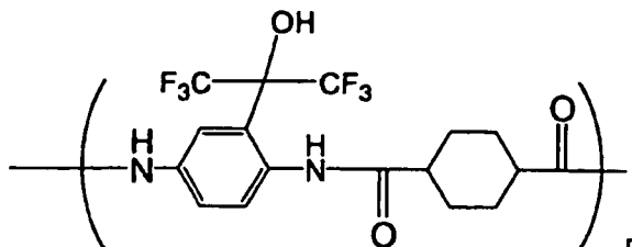
[Chem. 17]
