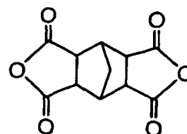
COMPOUND (f)
