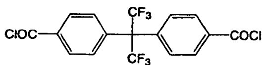
COMPOUND (c)
