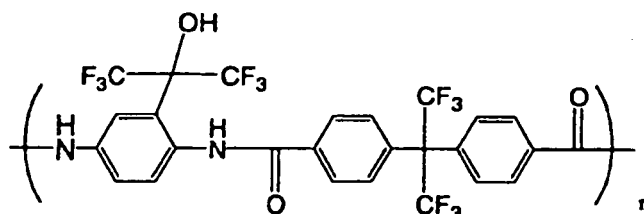
POLYMER (C)
