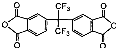
COMPOUND (e)
