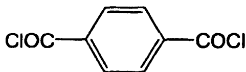
COMPOUND (a)
