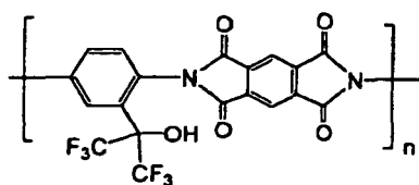
POLYMER (H)
