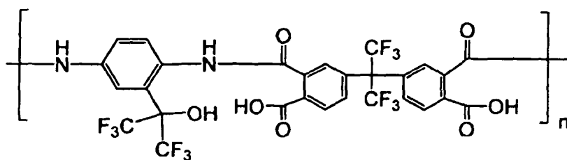
POLYMER (F)
