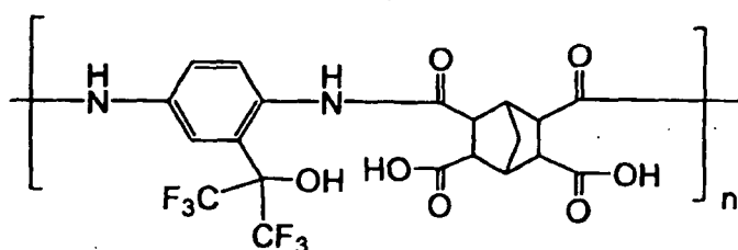
POLYMER (G)
