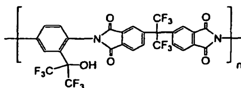
POLYMER (I)
