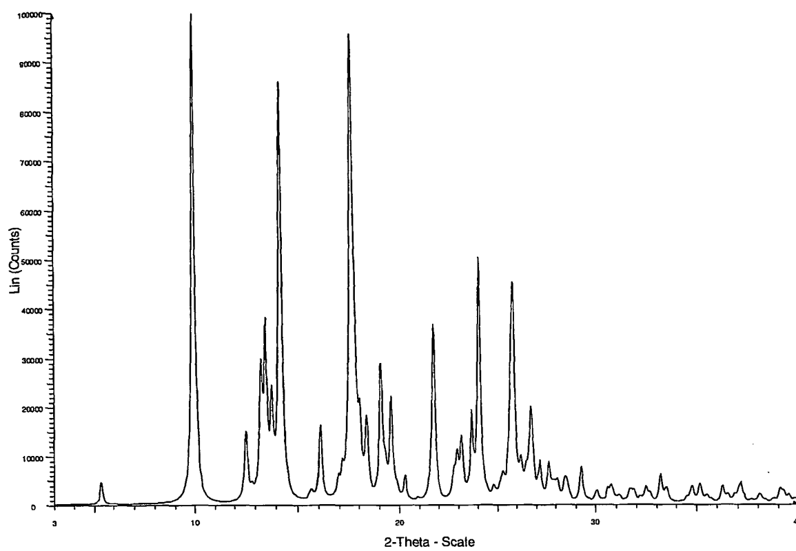
Figure 1a Form A calculated PXRD
