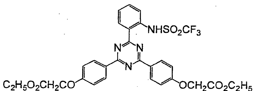
Comparative Compound (3)
