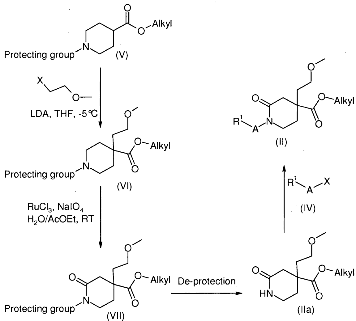
Scheme 2
