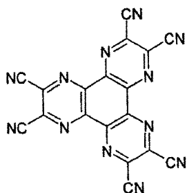
[Hexanitrile hexaazatriphenylene]
