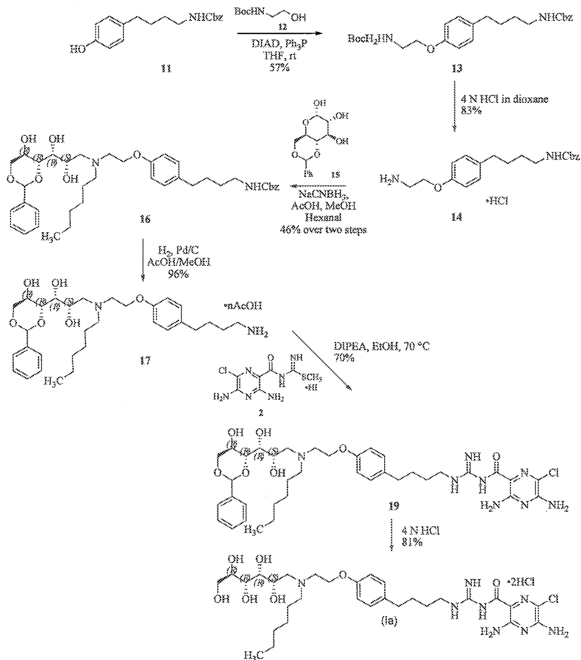
Scheme 2. Preparation of 3,5-Diamino-6-chloro- N -( N -(4-(2-(hexyl((2 S ,3 R ,4 R ,5 R )-2,3,4,5,6-pentahydroxyhexyl)amino)ethoxy)phenyl)butyl)carbamimidoyl)pyrazine-2-carboxamide
