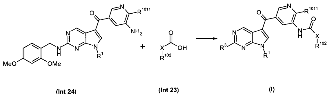
Scheme 11
