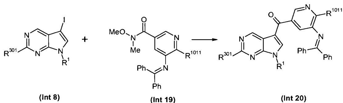
Scheme 7
