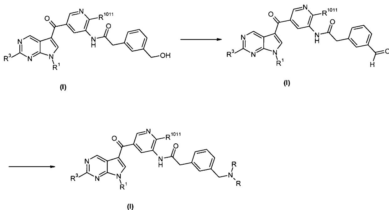
Scheme 14
