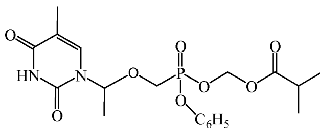
Compound (Ih)
