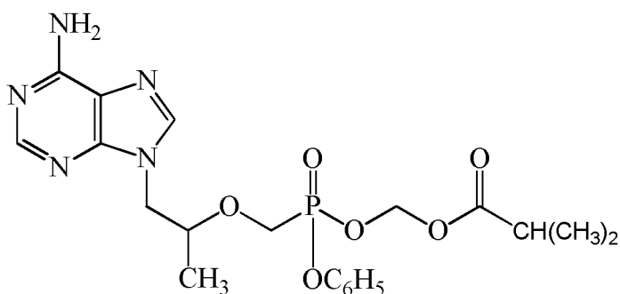
Compound (Ib)
