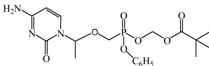
Compound (Ie)
