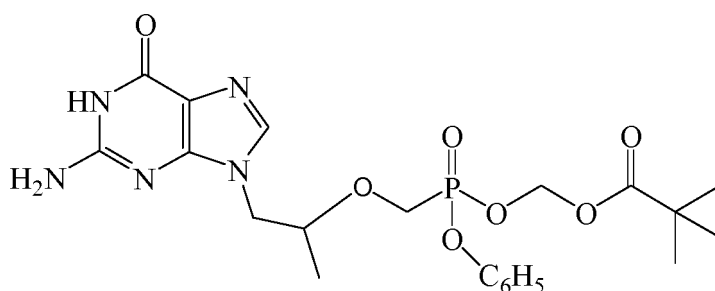
Compound (Ic)
