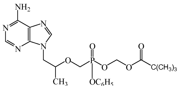
Compound (Ia)
