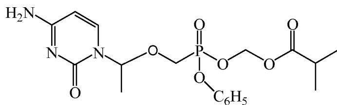
Compound (If)
