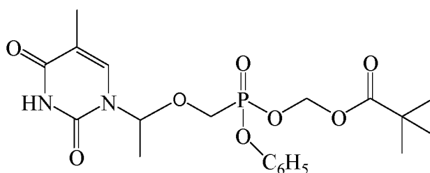
Compound (Ig)
