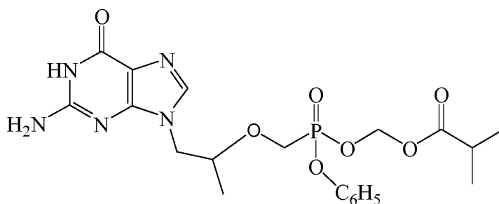
Compound (Id)
