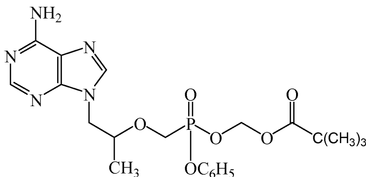
Formula Ia
