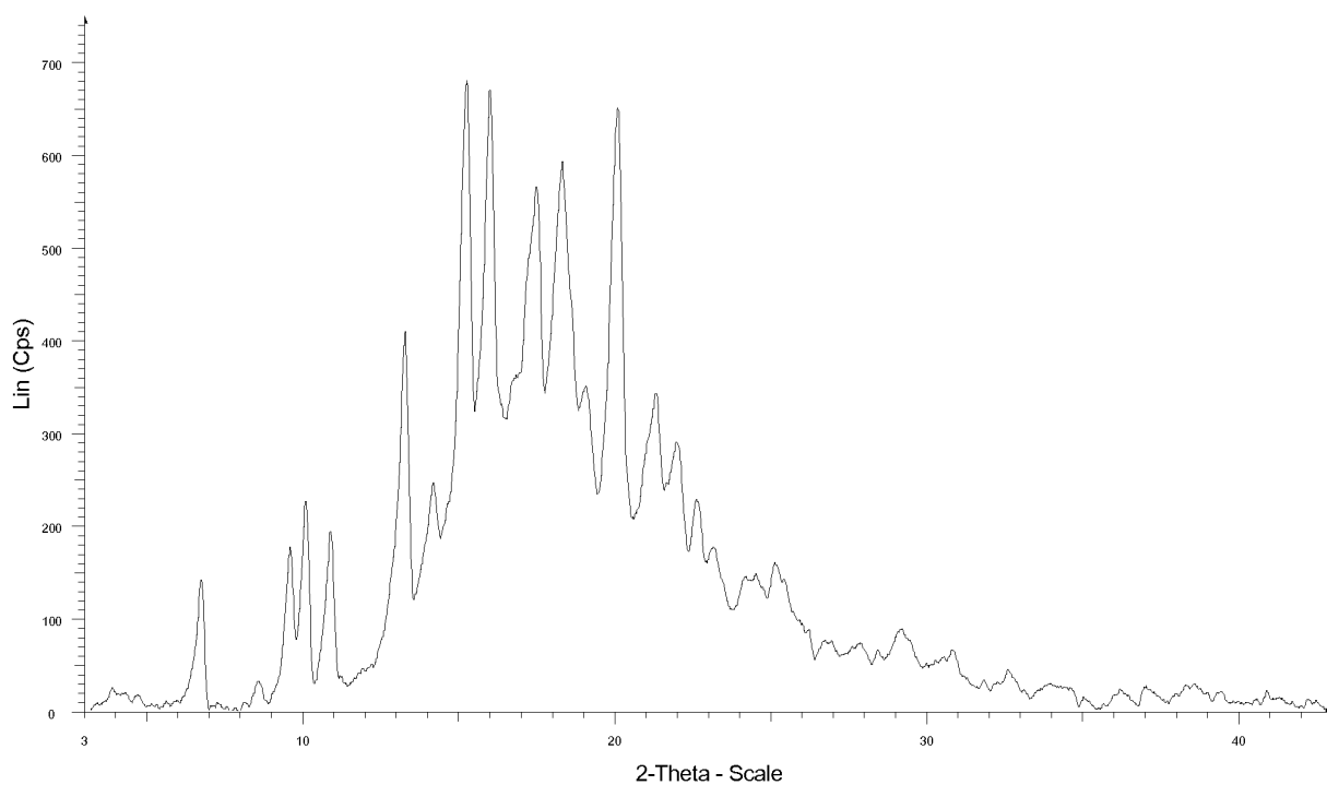
Fig. 2: X-ray powder spectrum of the product of example 3c:
