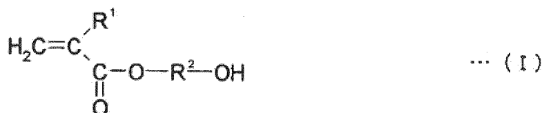
[Chemical formula 1]
