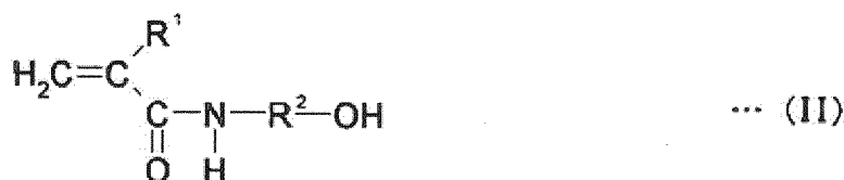
[Chemical formula 2]
