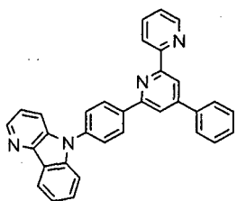
[Chem. 9]
