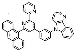
[Chem. 97]
