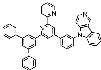
[Chem. 161]
