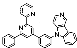
[Chem. 20]
