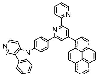
[Chem. 100]
