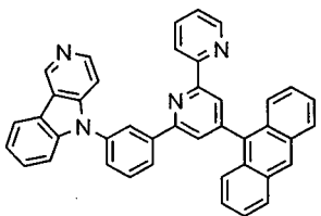
[Chem. 92]
