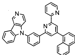
[Chem. 28]
