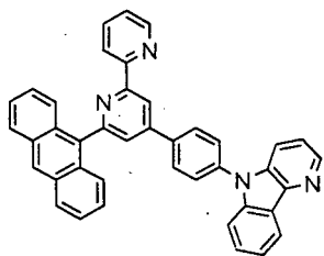
[Chem. 89]
