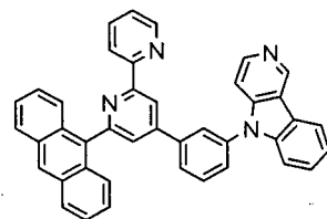
[Chem. 96]
