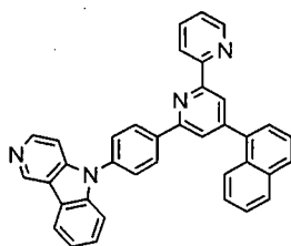
[Chem. 20]
