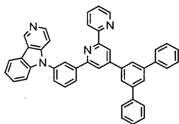
[Chem. 156]
