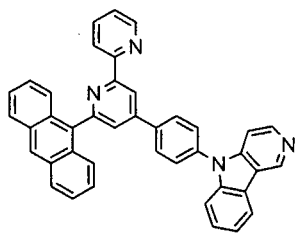
[Chem. 88]
