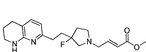
(S)-III
