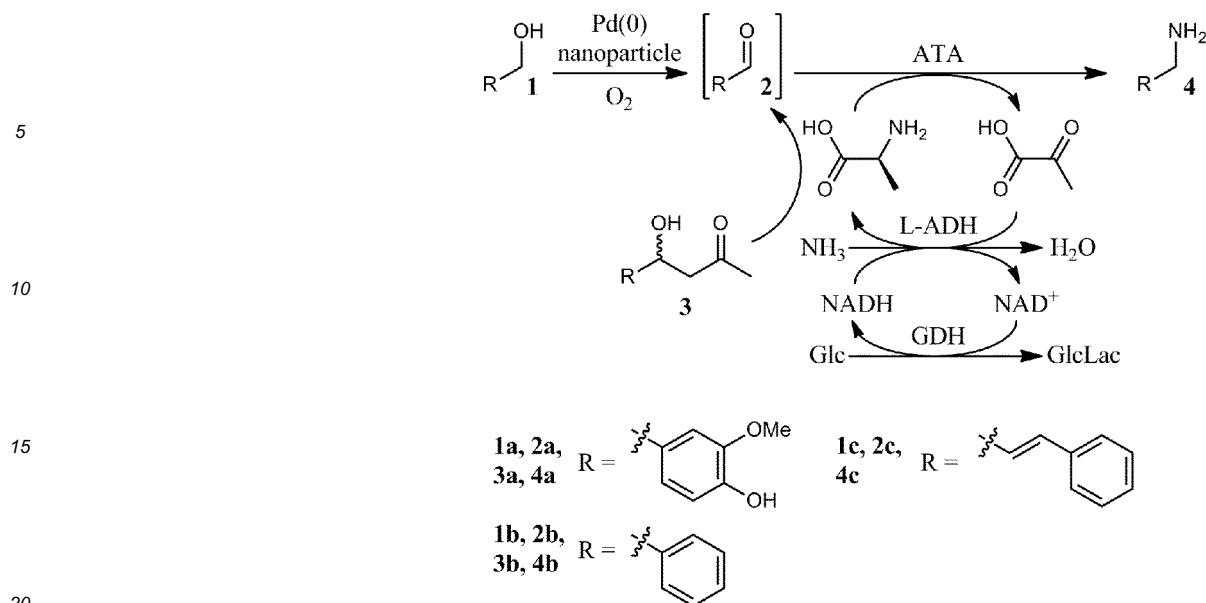
Scheme 3 – conversion of alcohols to amines and amides
