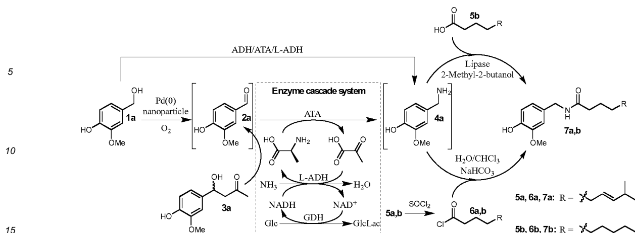
Scheme 4. Schematic overview of the total synthesis of capsaicin and nonivamide.
