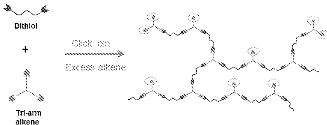
Scheme 1A – Polymer networks produced by thiol-ene click reaction containing surplus “clickable” functional groups (alkene).
