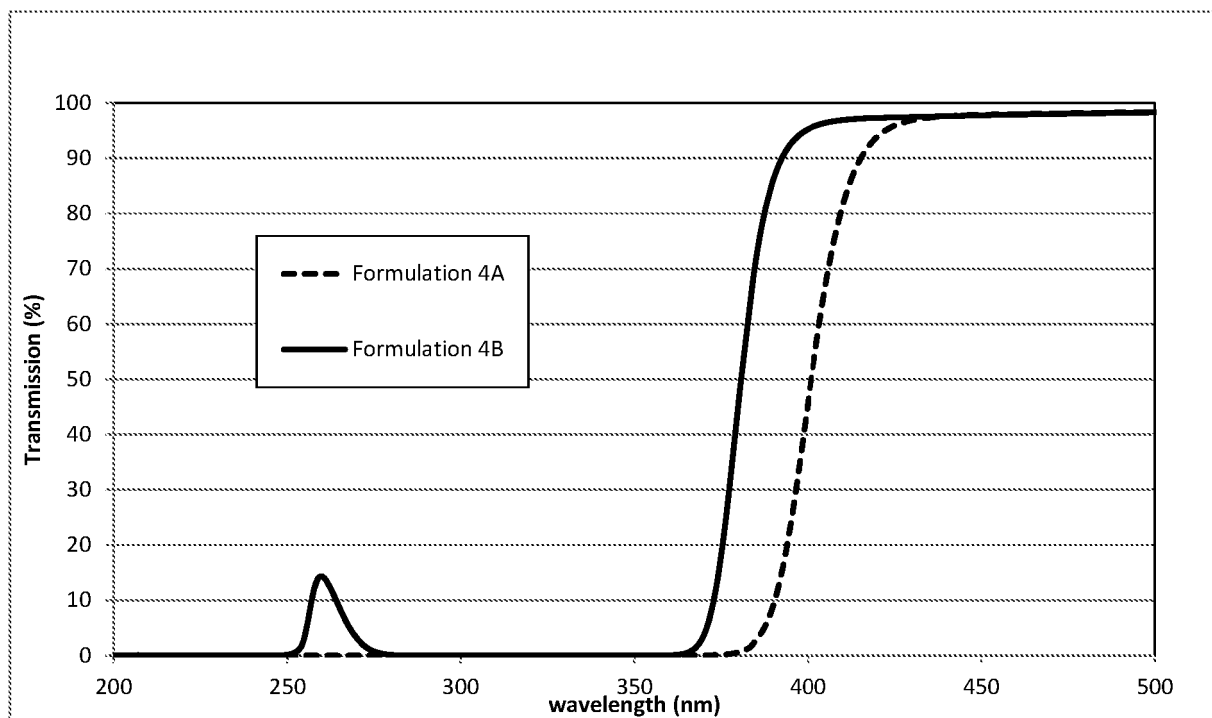
FIG. 3 –Transmission Spectra of Contact Lenses made from Silicone Hydrogel Formulation 4A containing 0.619 mole percent of Compound (M) and Silicone Hydrogel Formulation 4B containing 0.619 mole percent of Norbloc® in borate packaging solutions
