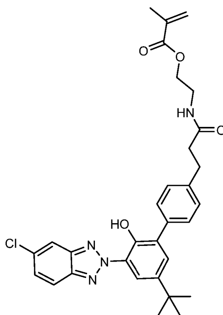
2-(3-(5'-(tert-butyl)-3'-(5-chloro-2H-benzo[d][1,2,3]triazol-2-yl)-2'-hydroxy-[1,1'-biphenyl]-4-yl)propanamido)ethyl methacrylate (Compound M)
