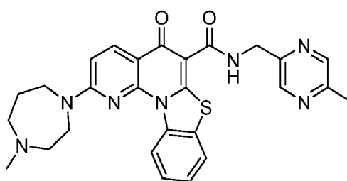
Compound I
