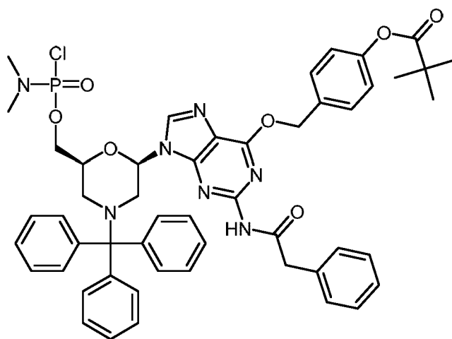
Compound (E1)
