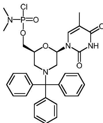
Compound (G1)
