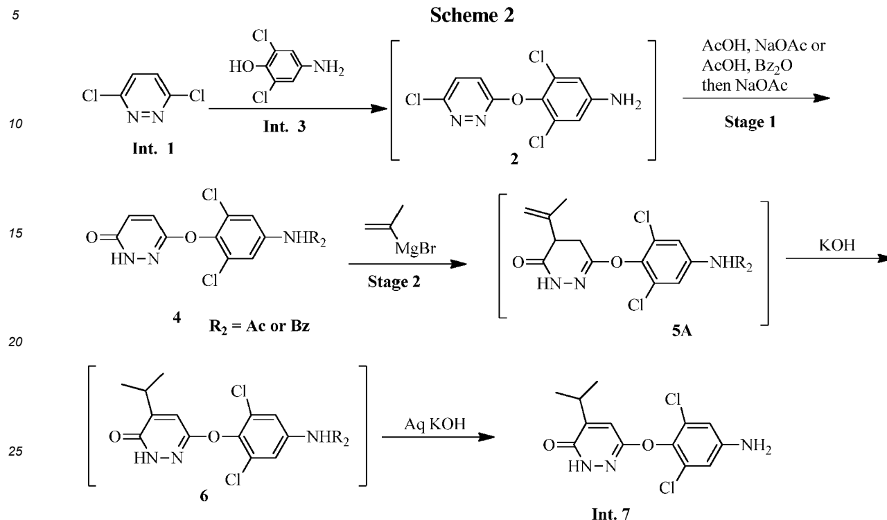
Scheme 2: Synthesis of 6-(4-amino-2,6-dichlorophenoxy)-4-isopropylpyridazin-3(2H)-one ( Int. 7 ) with isopropenyl Grignard reagent.
