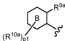
[Chemical Formula 21]
