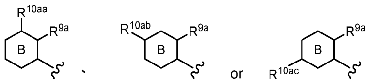
[Chemical Formula 54]
