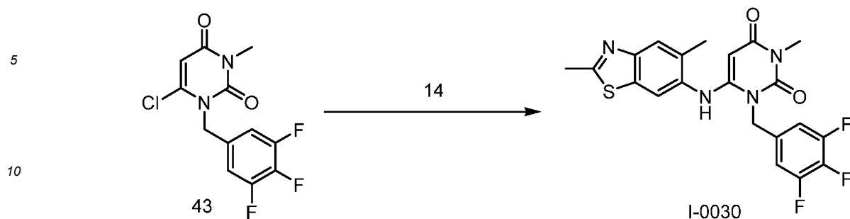
[Chemical Formula 126]
