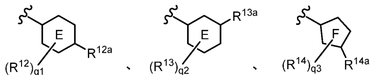
[Chemical Formula 78]
