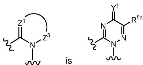
[Chemical Formula 25]
