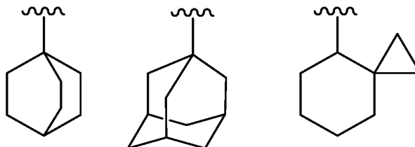
[Chemical Formula 29]
