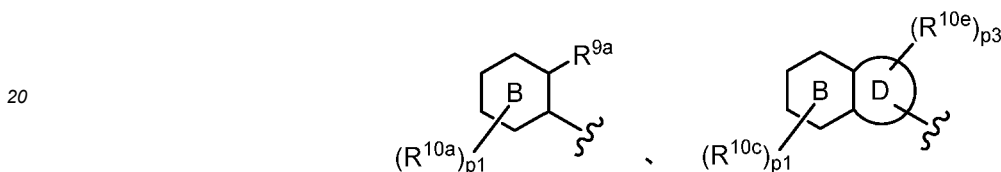
[Chemical Formula 73]
