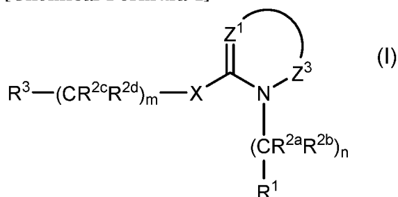
[Chemical Formula 1]
