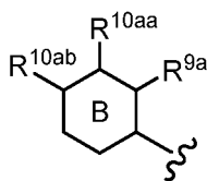
[Chemical Formula 53]
