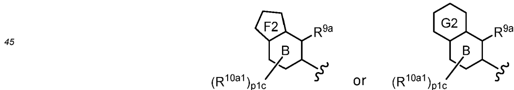
[Chemical Formula 62]
