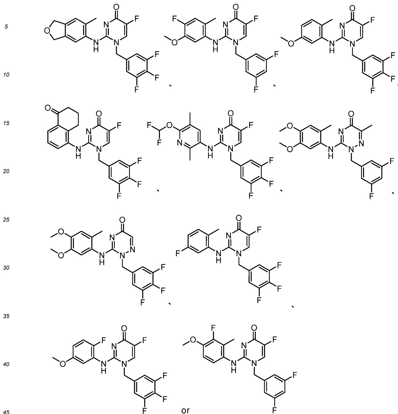
[Chemical Formula 27]
