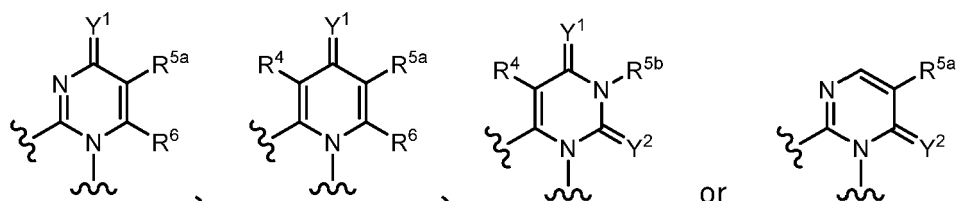
[Chemical Formula 14]
