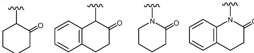
[Chemical Formula 32]
