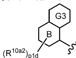
[Chemical Formula 68]
