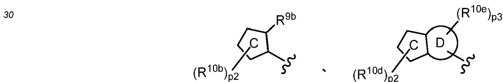
[Chemical Formula 74]
