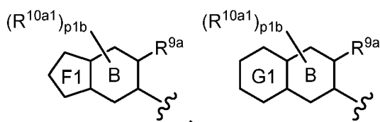
[Chemical Formula 79]
