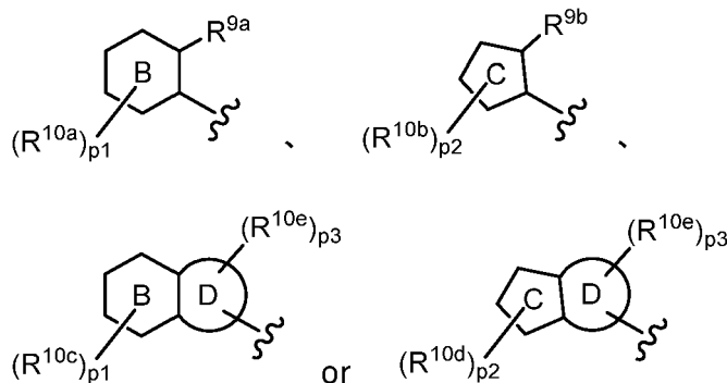
[Chemical Formula 8]
