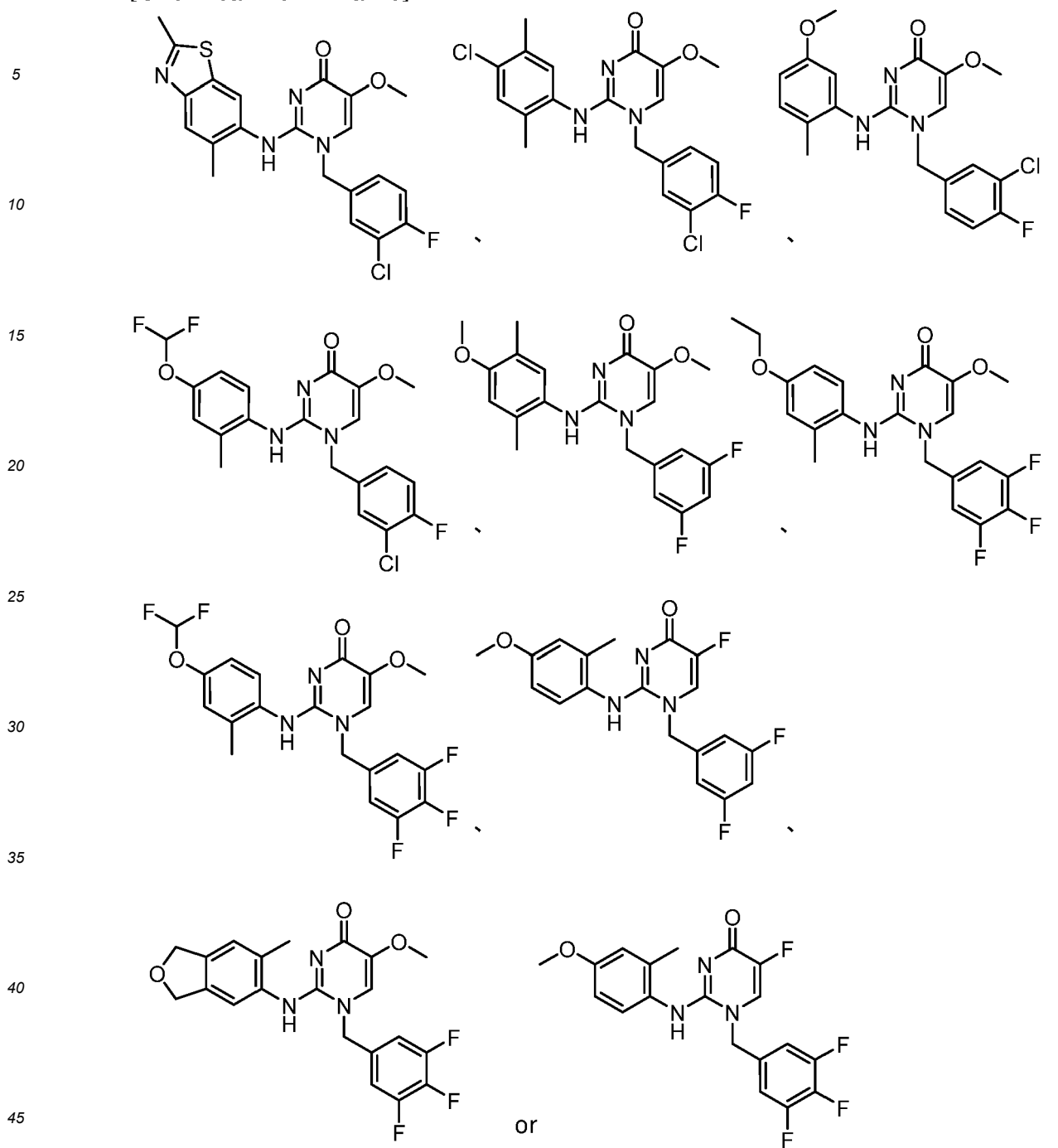
[Chemical Formula 26]
