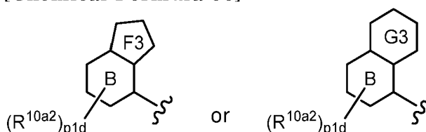
[Chemical Formula 66]
