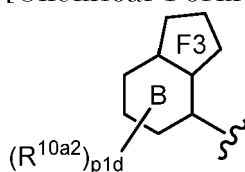
[Chemical Formula 67]
