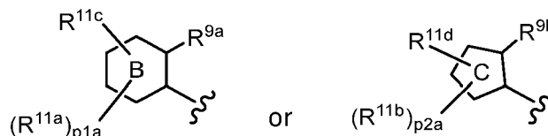
[Chemical Formula 18]
