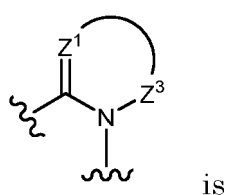
[Chemical Formula 2]
