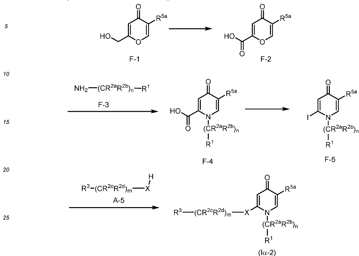
[Chemical Formula 87]
