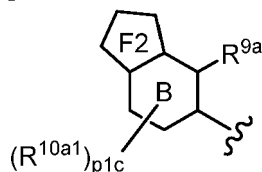
[Chemical Formula 63]
