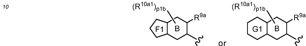
[Chemical Formula 59]
