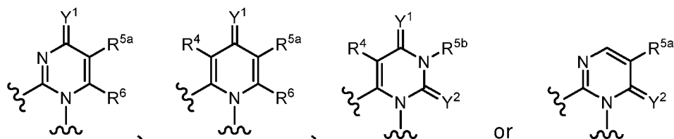
[Chemical Formula 23]
