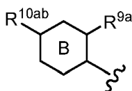
[Chemical Formula 56]
