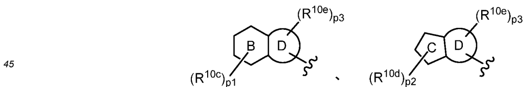
[Chemical Formula 75]
