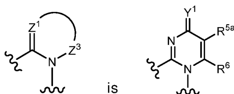
[Chemical Formula 15]
