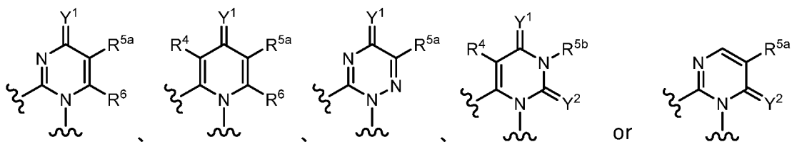
[Chemical Formula 20]
