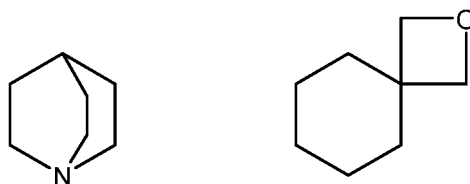
[Chemical Formula 30]
