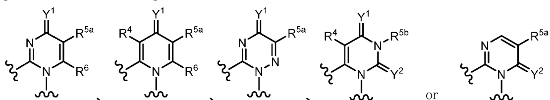
[Chemical Formula 14]
