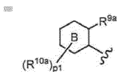
[Chemical Formula 12]
