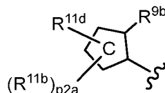
[Chemical Formula 77]
