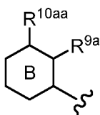
[Chemical Formula 55]
