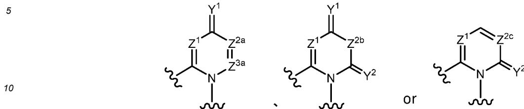
[Chemical Formula 72]
