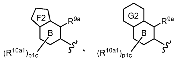
[Chemical Formula 80]
