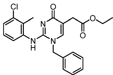
[Chemical Formula 122]
