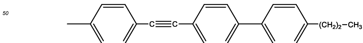
L(16) 4-(biphenyl-4-carbonyloxy)-piperidin-1-yl
