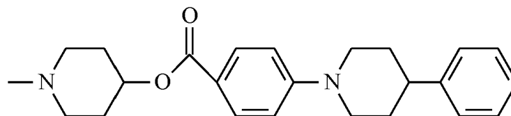
L(20) 4-butyl-[1,1';4',1'']terphenyl-4-yl
