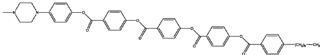
L(12) 4-(4'-Propylbiphenyl-4-ylethynyl)phenyl
