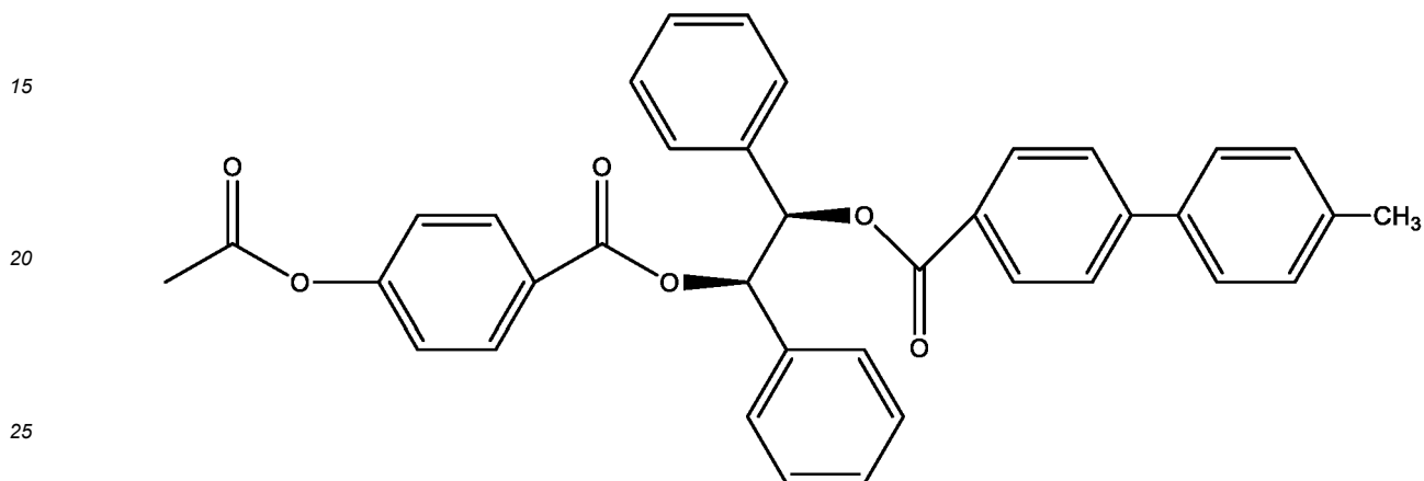
L(10) 4-[4-(4-[4-[3-(6-[4-[4-(4-nonyl-benzoyloxy)-phenoxy]-hexyloxycarbonyl]-propionyloxy]-benzoyloxy)-benzoyloxy)-phenyl]-piperazin-1-yl
