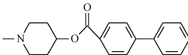
L(18) 4-(4-phenylcarbamoyl-phenylcarbamoyl)-piperidin-1-yl
