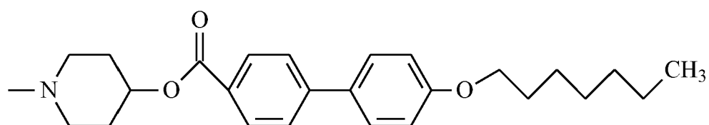
L(28) 4-(4'-hexyloxy-biphenyl-4-carbonyloxy)-piperidin-1-yl
