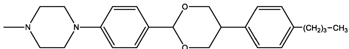
L(33) 1-[4-[5-(4-butyl-phenyl)-[1,3]dioxan-2-yl]-phenyl]-4-methyl-piperazin-1-yl
