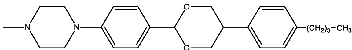
L(34) 4-(7-(4-propylphenylcarbonyloxy)bicyclo[3.3.0]oct-2-yl)oxycarbonyl)phenyl
