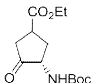
(3R)-ethyl-3-((tert-butoxycarbonyl)amino)-4-oxo-cyclopentane carboxylate (12)
