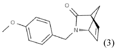
(1 R ,4 S )-2-(4-Methoxybenzyl)-2-azabicyclo[2.2.1]hept-5-en-3-one (3)
