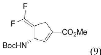
Methyl ( S )-3-((tert-butoxycarbonyl)amino)-4-(difluoromethylene)cyclopent-1-ene-1-carboxylate (9)
