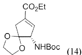
Ethyl (S)-9-(tert-butoxycarbonylamino)-1,4-dioxo-7-spiro[4.4]nonene-7-carboxylate (14)
