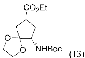
Ethyl (9S)-9-(tert-butoxycarbonylamino)-1,4-dioxo-7-spiro[4.4]nonanecarboxylate (13)
