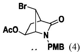
(1 R ,4 R ,6 S ,7 R )-7-Bromo-2-(4-methoxybenzyl)-3-oxo-2-azabicyclo[2.2.1]heptan-6-yl acetate (4)
