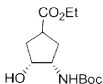
(3R,4S)-ethyl-3-((tert-butoxycarbonyl)amino)-4-(hydroxy)cyclopentane carboxylate (11)
