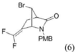
(1 R ,4 R ,7 R )-7-Bromo-6-(difluoromethylene)-2-(4-methoxybenzyl)-2-azabicyclo[2.2.1]heptan-3-one (6)
