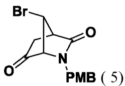
(1 R ,4 R ,7 R )-7-Bromo-2-(4-methoxybenzyl)-2-azabicyclo[2.2.1]heptane-3,6-dione (5)
