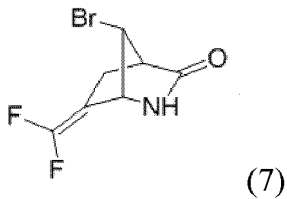
(1 R ,4 R ,7 R )-7-Bromo-6-(difluoromethylene)-2-azabicyclo[2.2.1]heptan-3-one (7)
