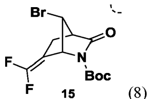
(1 R ,4 R ,7 R )-7-Bromo-6-(difluoromethylene)-2-(tert-butoxycarbonyl)-2-azabicyclo[2.2.1]heptan-3-one (8)
