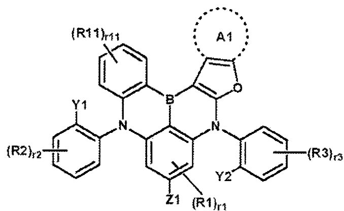
[Chemical Formula 6]
