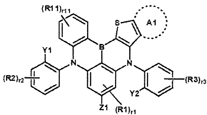
[Chemical Formula 6]
