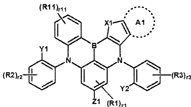
[Chemical Formula 3]
