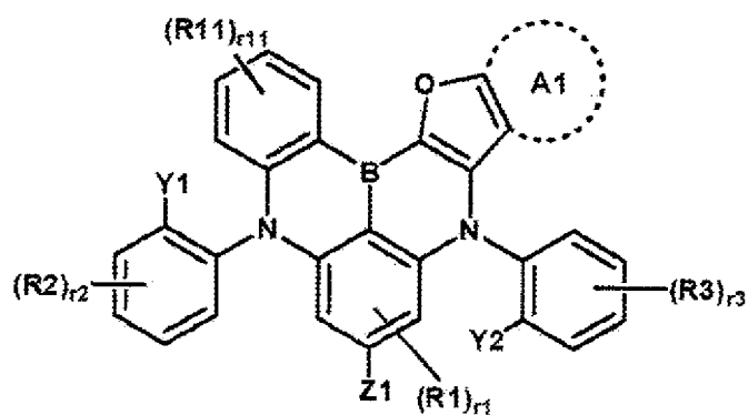
[Chemical Formula 5]
