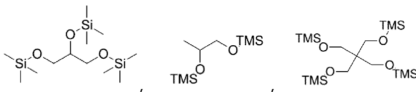
1,2-bis(trimethylsilyloxy)-dodecane,
