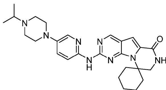
Compound 1
