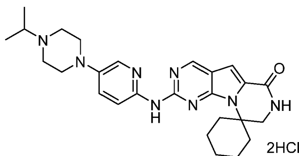
Compound 2
