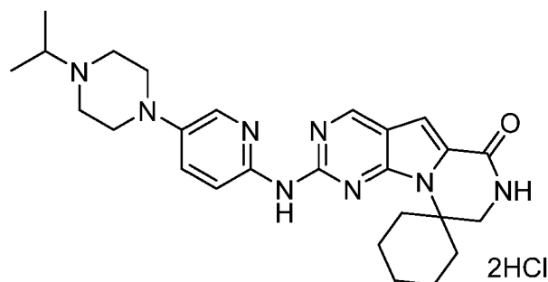
Compound 2
