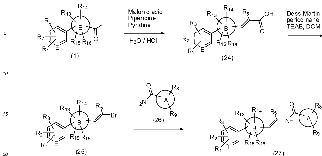
Scheme 7
