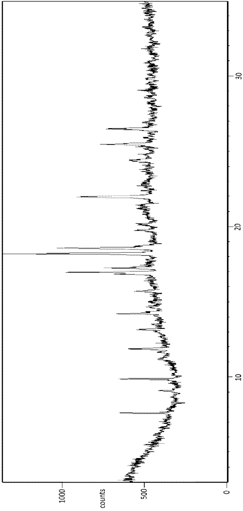
Degrees 2-theta
