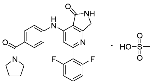
Compound 1M
