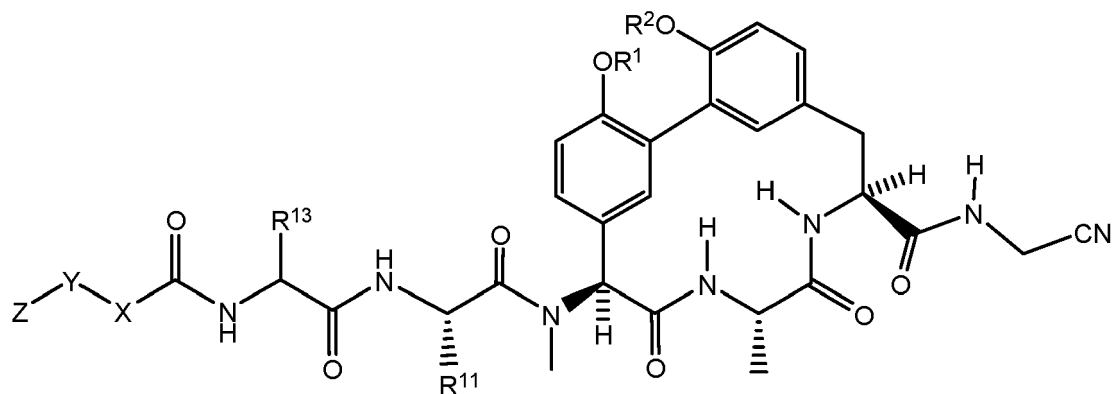
Formula (IIc);
