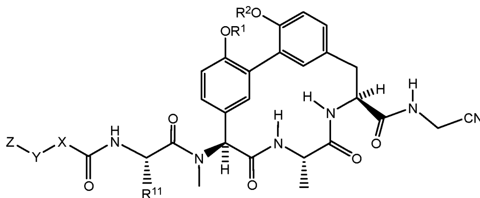
Formula (IVc);
