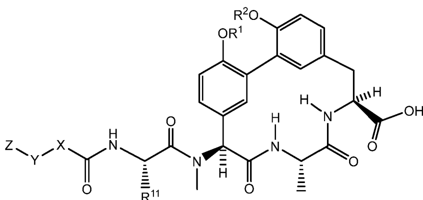
Formula (Vc);
