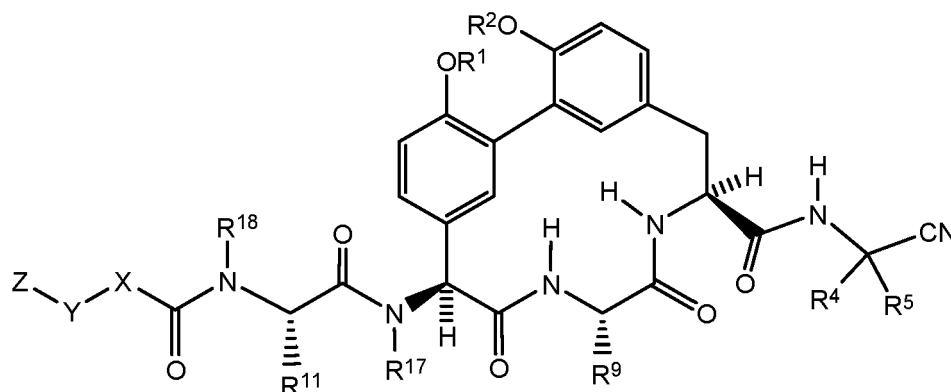
Formula (IVb);
