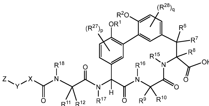
Formula (V);
