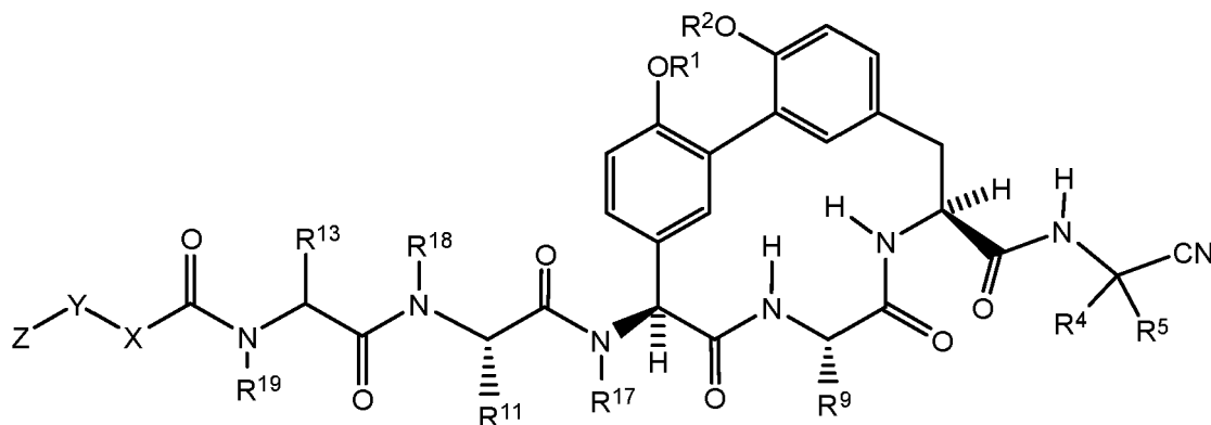
Formula (IIb);
