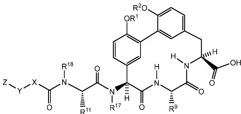
Formula (Vb);
