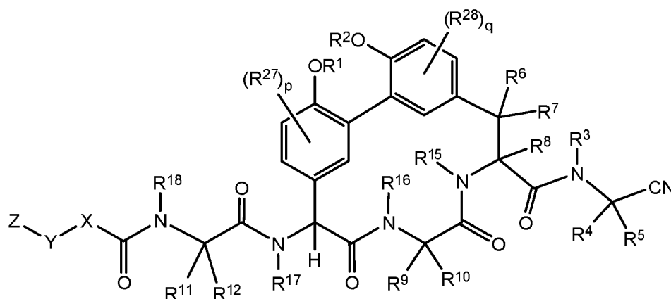
Formula (IV);
