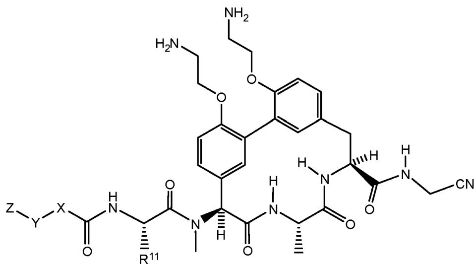
Formula (Id):
