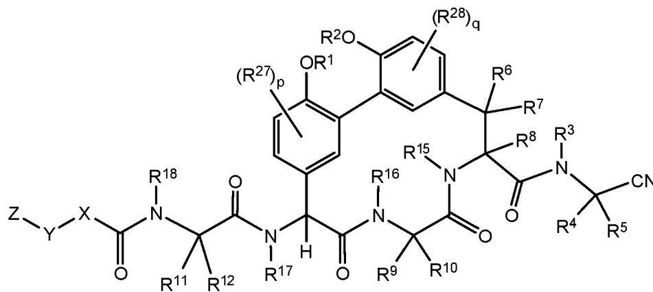
Formula (III);
