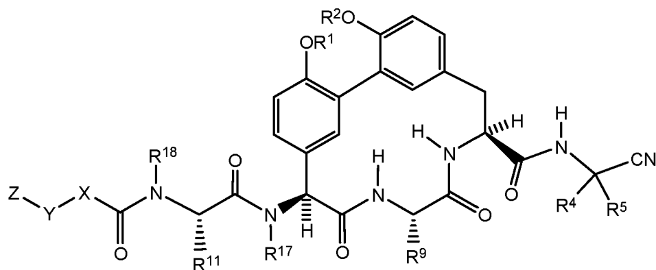
Formula (IIIb);
