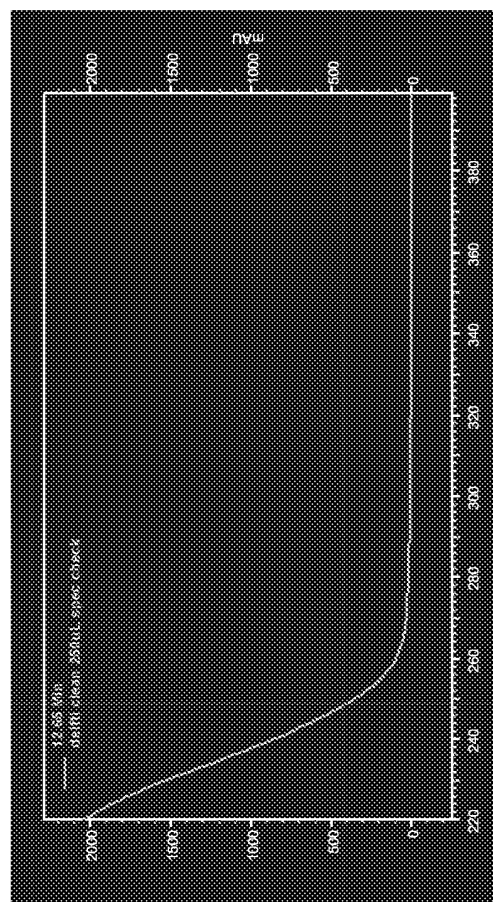
Main isomer 12.6min 70%
