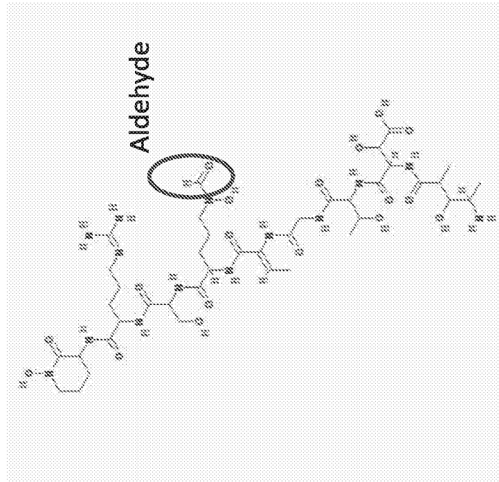
Delftibactin A
