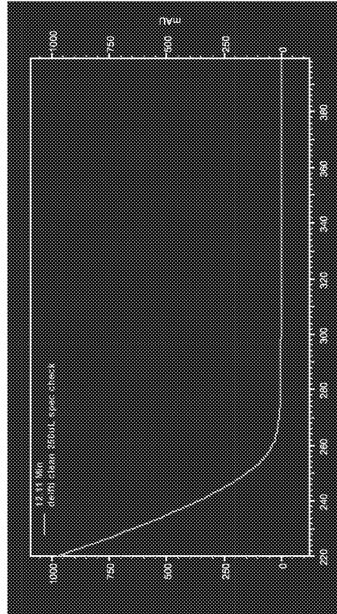
Secondary isomer 12.1min 30%
