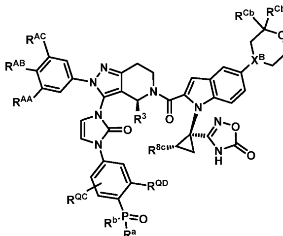
Formula (S, S, S)-(IE)
