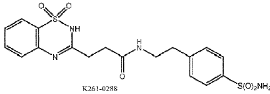
10 3-(1,1-dioxido-2H-benzo[e][1,2,4]thiadiazin-3-yl)-N-(4-sulfamoylphenethyl)propanamide
