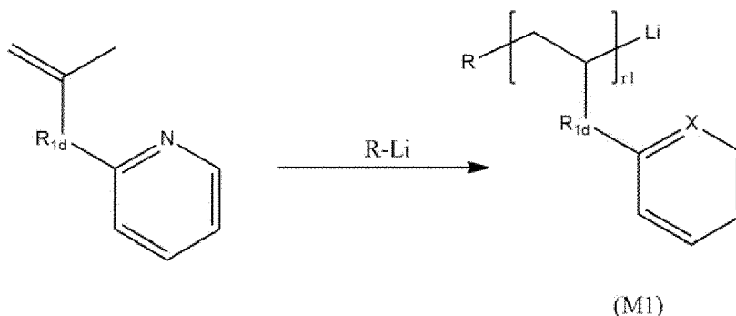
[Reaction 1]
